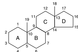
Figure 14–14. The steroid nucleus.
