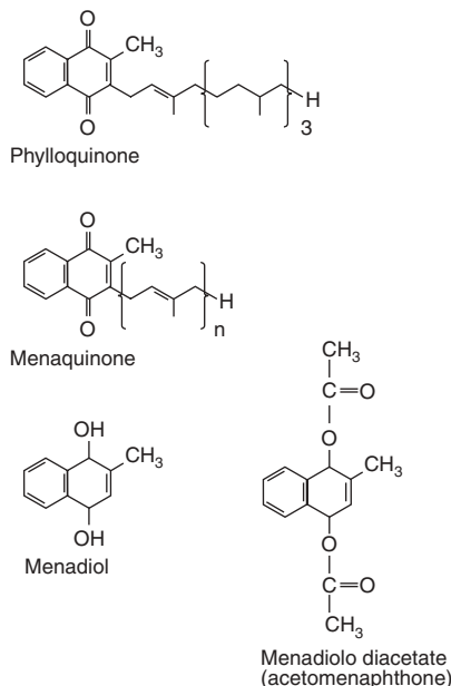
Figure 45-7. The vitamin K vitamins. Menadiol (or menadione) and menadiolo diacetate are synthetic compounds that are converted to menaquinone in the liver and have vitamin K activity.
