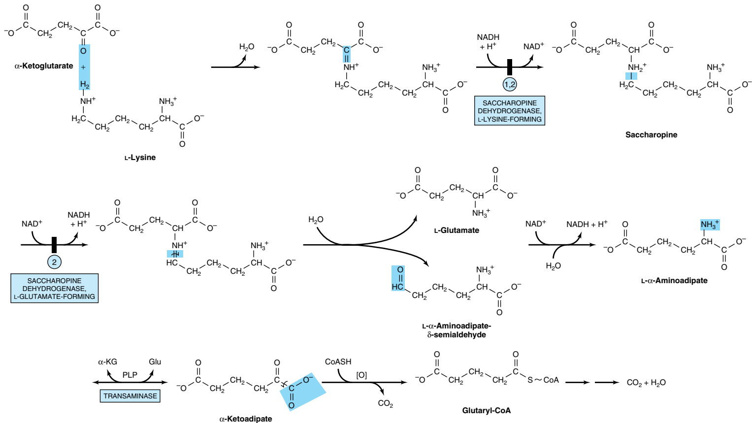
Figure 30–14. Catabolism of L-lysine. (α-KG, α-ketoglutarate; Glu, glutamate; PLP, pyridoxal phosphate.) Circled numerals indicate the probable sites of the metabolic defects in ① periodic hyperlysinemia with associated hyperammonemia; and ② persistent hyperlysinemia without associated hyperammonemia.
