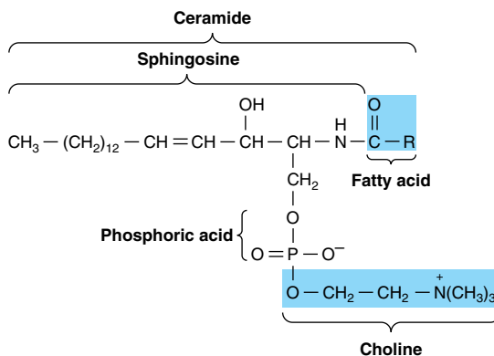
Figure 14–11. A sphingomyelin.
