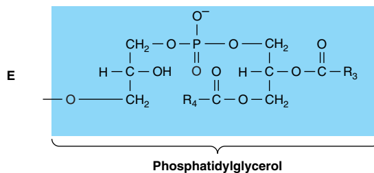
Figure 14–8. Phosphatidic acid and its derivatives. The O − shown shaded in phosphatidic acid is substituted by the substituents shown to form in (A) 3-phosphatidylcholine, (B) 3-phosphatidylethanolamine, (C) 3-phosphatidylserine, (D) 3-phosphatidylinositol, and (E) cardiolipin (diphosphatidylglycerol).
