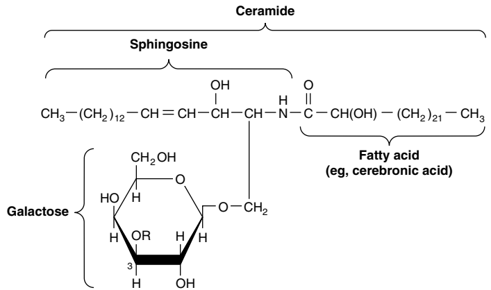
Figure 14–12. Structure of galactosylceramide (galactocerebroside, R = H), and sulfogalactosylceramide (a sulfatide, R = \text{SO}_4^{2-} ).
