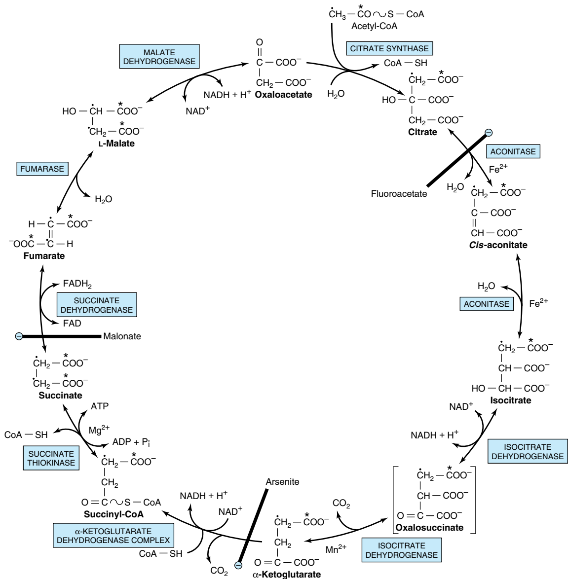
Figure 16-3. Reactions of the citric acid (Krebs) cycle. Oxidation of \text{NADH} and \text{FADH}_2 in the respiratory chain leads to the generation of ATP via oxidative phosphorylation. In order to follow the passage of acetyl-CoA through the cycle, the two carbon atoms of the acetyl radical are shown labeled on the carboxyl carbon (designated by asterisk) and on the methyl carbon (using the designation *). Although two carbon atoms are lost as \text{CO}_2 in one revolution of the cycle, these atoms are not derived from the acetyl-CoA that has immediately entered the cycle but from that portion of the citrate molecule that was derived from oxaloacetate. However, on completion of a single turn of the cycle, the oxaloacetate that is regenerated is now labeled, which leads to labeled \text{CO}_2 being evolved during the second turn of the cycle. Because succinate is a symmetric compound and because succinate dehydrogenase does not differentiate between its two carboxyl groups, "randomization" of label occurs at this step such that all four carbon atoms of oxaloacetate appear to be labeled after one turn of the cycle. During gluconeogenesis, some of the label in oxaloacetate is incorporated into glucose and glycogen (Figure 19-1). For a discussion of the stereochemical aspects of the citric acid cycle, see Greville (1968). The sites of inhibition ( \ominus ) by fluoroacetate, malonate, and arsenite are indicated.
