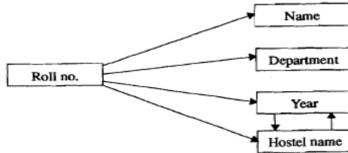
Figure 6: Dependency diagram for the relation
