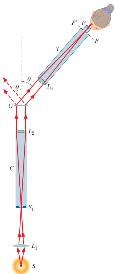
Figure 36-23 A simple type of grating spectroscopy used to analyze the wavelengths of light emitted by source S .
