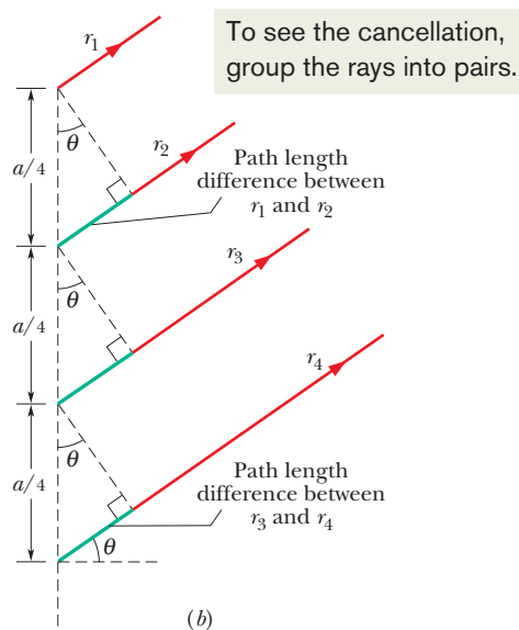
Figure 36-6 (a) Waves from the top points of four zones of width a/4 undergo fully destructive interference at point P_2 . (b) For D \gg a , we can approximate rays r_1 , r_2 , r_3 , and r_4 as being parallel, at angle \theta to the central axis.
