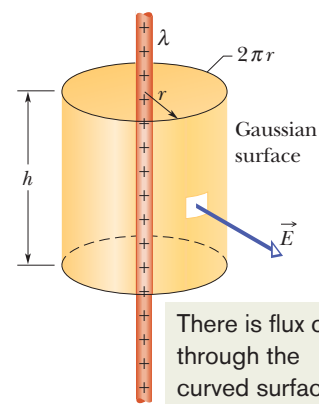
Figure 23-14 A Gaussian surface in the form of a closed cylinder surrounds a section of a very long, uniformly charged, cylindrical plastic rod.
