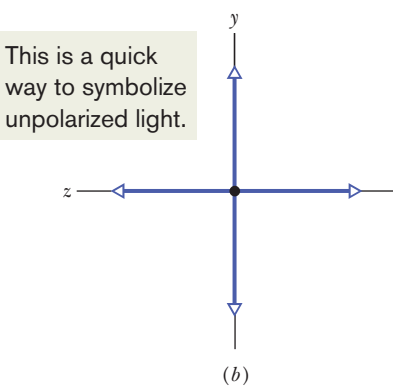
Figure 33-10 (a) Unpolarized light consists of waves with randomly directed electric fields. Here the waves are all traveling along the same axis, directly out of the page, and all have the same amplitude E . (b) A second way of representing unpolarized light—the light is the superposition of two polarized waves whose planes of oscillation are perpendicular to each other.
