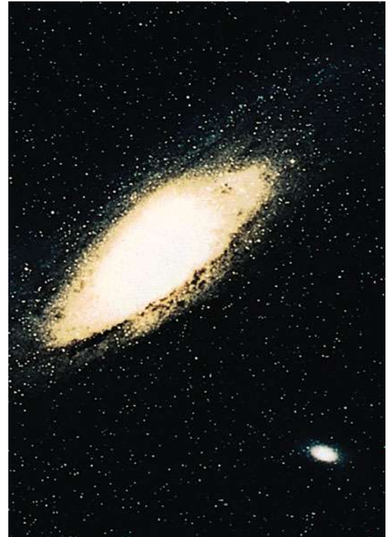
Figure 13-1 The Andromeda Galaxy. Located 2.3 \times 10^6 light-years from us, and faintly visible to the naked eye, it is very similar to our home galaxy, the Milky Way.
