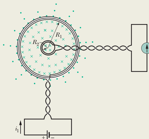
Figure 30-20 A small coil is located at the center of a large coil. The mutual inductance of the coils can be determined by sending current i_1 through the large coil.
