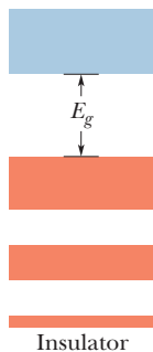
Figure 41-4 The band-gap pattern for an insulator; filled levels are shown in red and empty levels in blue.
