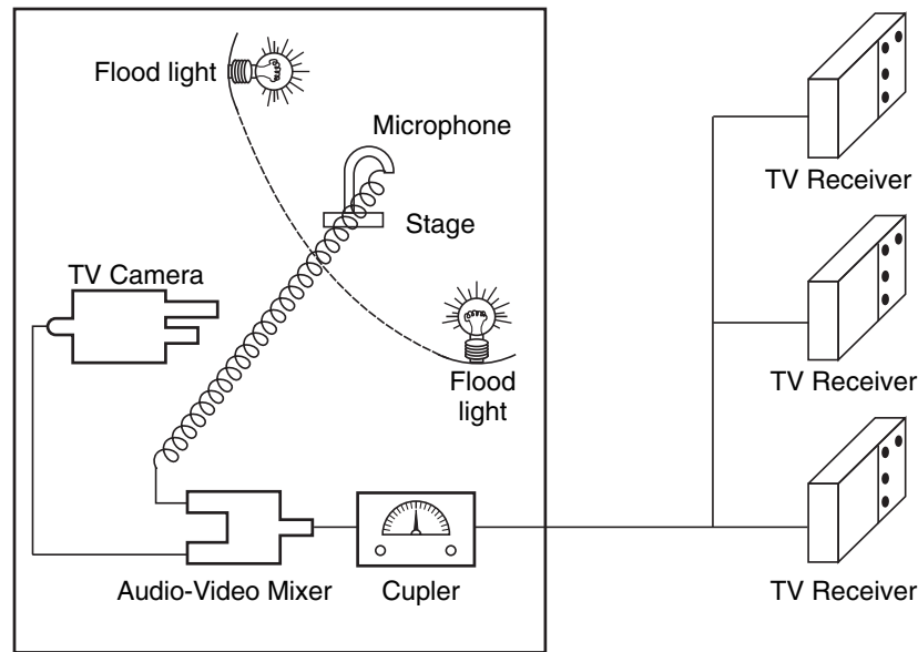
Fig. Simple closed circuit TV system
