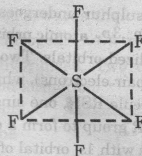
Fig. 2.19 Octahedral shape of SF_6 molecule
