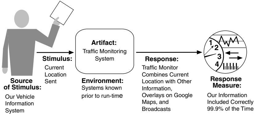
Sample concrete interoperability scenario
