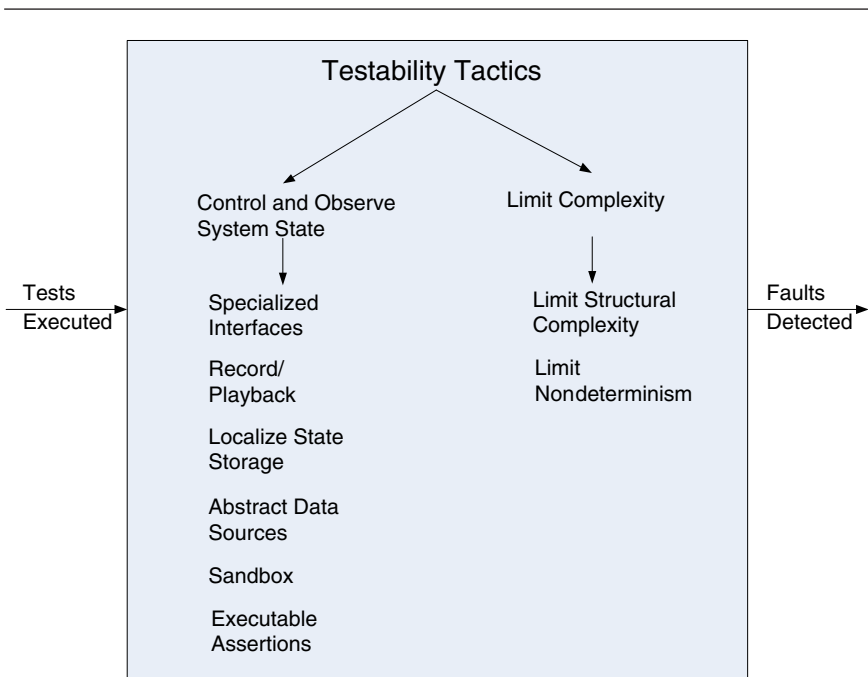
FIGURE 10.4 Testability tactics
