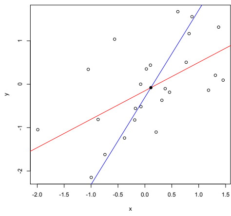
Figure 3.11: Plot of two regression lines. Notice that they cross at (\bar{x}, \bar{y}) .
