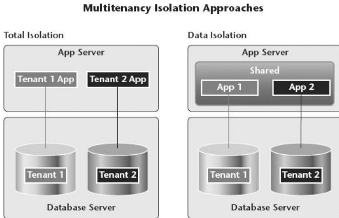
Figure 8.2 Data Segregation
