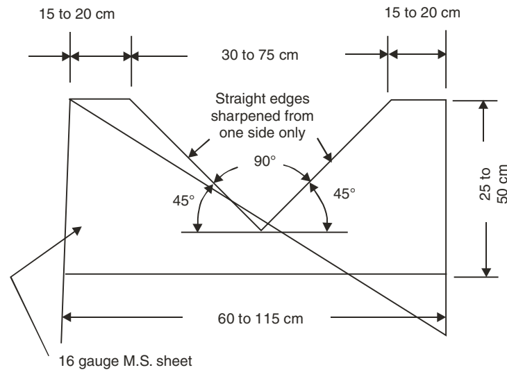
Fig. 11.12 Triangular weir
