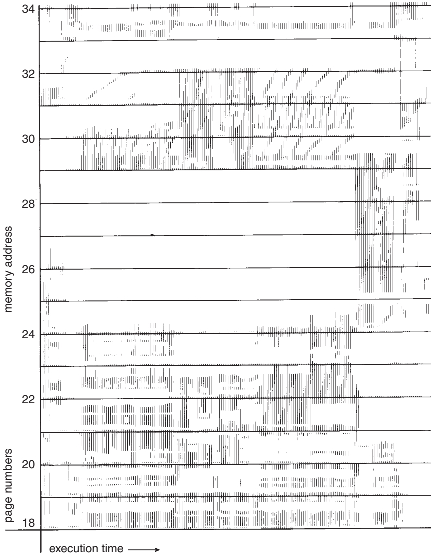
Figure 8.19 Locality in a memory-reference pattern.
