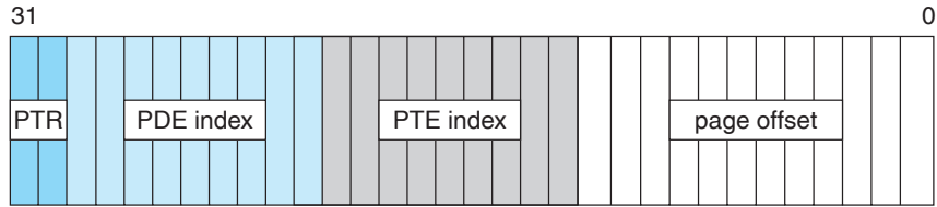
Figure 16.4 Virtual-to-physical address translation on IA32.
