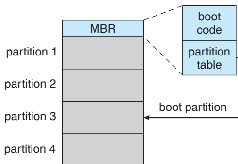
Figure 11.9 Booting from disk in Windows.
