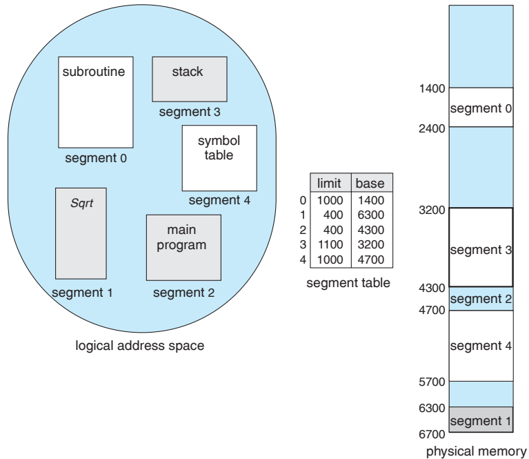
Figure 7.20 Example of segmentation.
