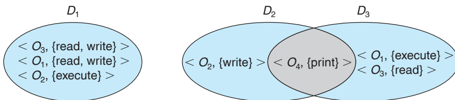
Figure 13.1 System with three protection domains.
