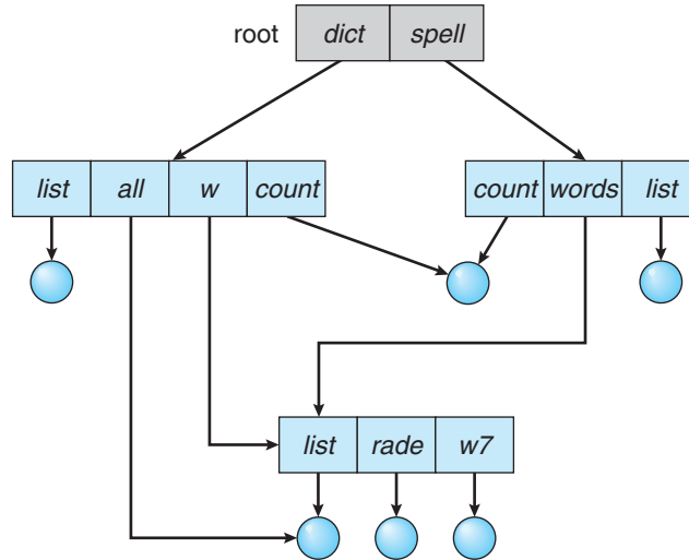
Figure 9.11 Acyclic-graph directory structure.
