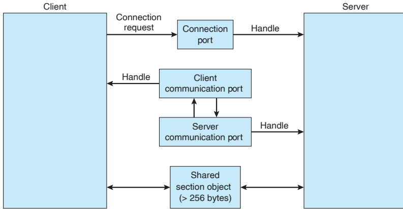
Figure 3.17 Local procedure calls in Windows.
