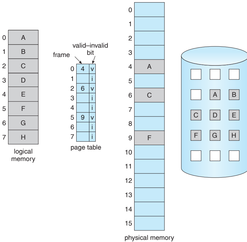
Figure 8.5 Page table when some pages are not in main memory.
