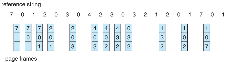
Figure 8.15 LRU page-replacement algorithm.
