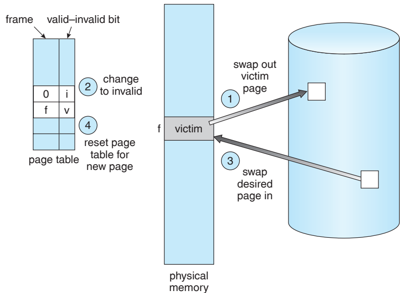
Figure 8.10 Page replacement.
