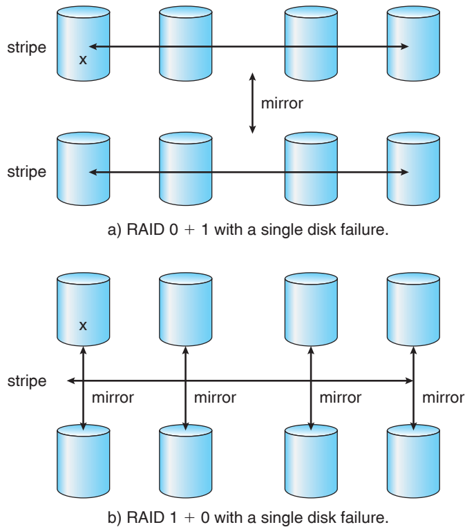
Figure 11.12 RAID 0 + 1 and 1 + 0.
