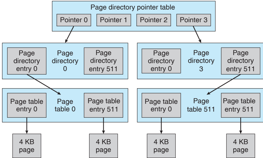
Figure 16.3 Page-table layout.
