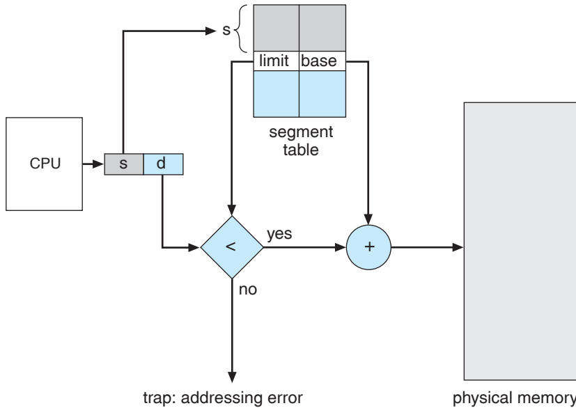
Figure 7.19 Segmentation hardware.
