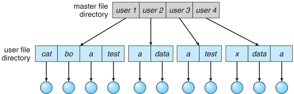
Figure 9.9 Two-level directory structure.
