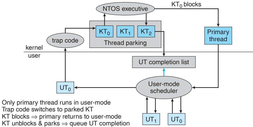
Figure 16.11 User-mode scheduling.
