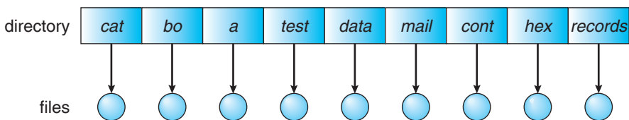
Figure 9.8 Single-level directory.
