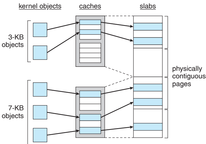
Figure 8.28 Slab allocation.
