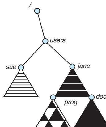
Figure 9.14 Mount point.
