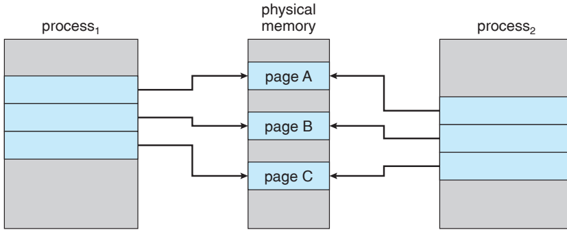
Figure 8.7 Before process 1 modifies page C.
