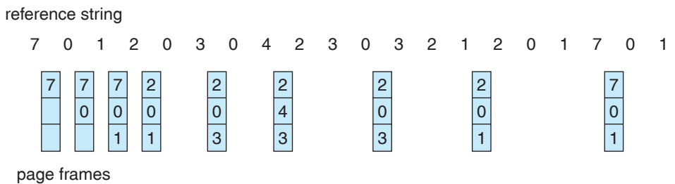
Figure 8.14 Optimal page-replacement algorithm.
