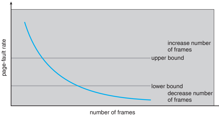
Figure 8.21 Page-fault frequency.
