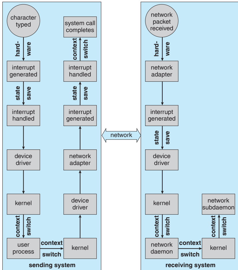
Figure 12.15 Intercomputer communications.
