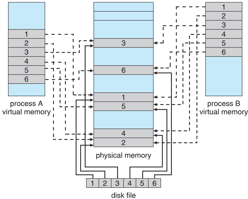
Figure 8.23 Memory-mapped files.
