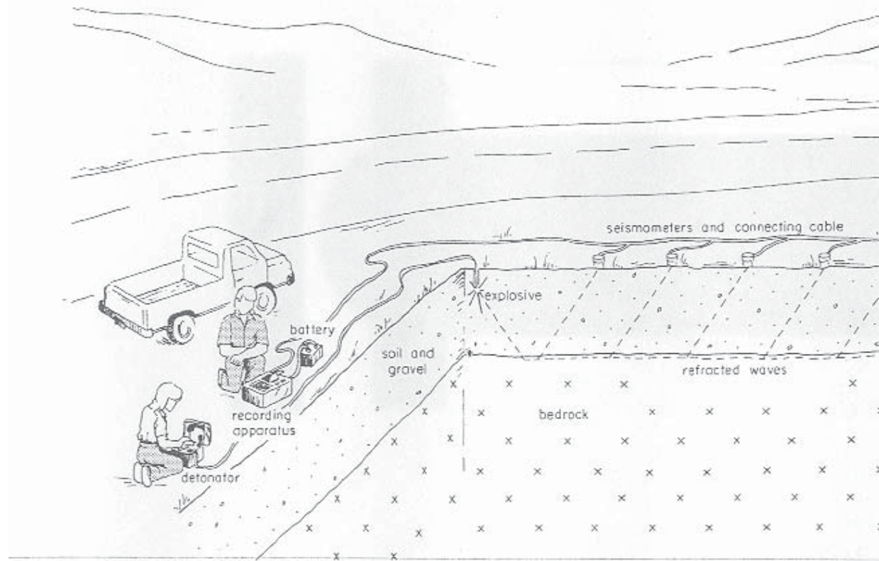
Figure 1-2 Seismic refraction experiment to measure the thickness of soil and gravel that covers solid bedrock. The times required for refracted waves to
