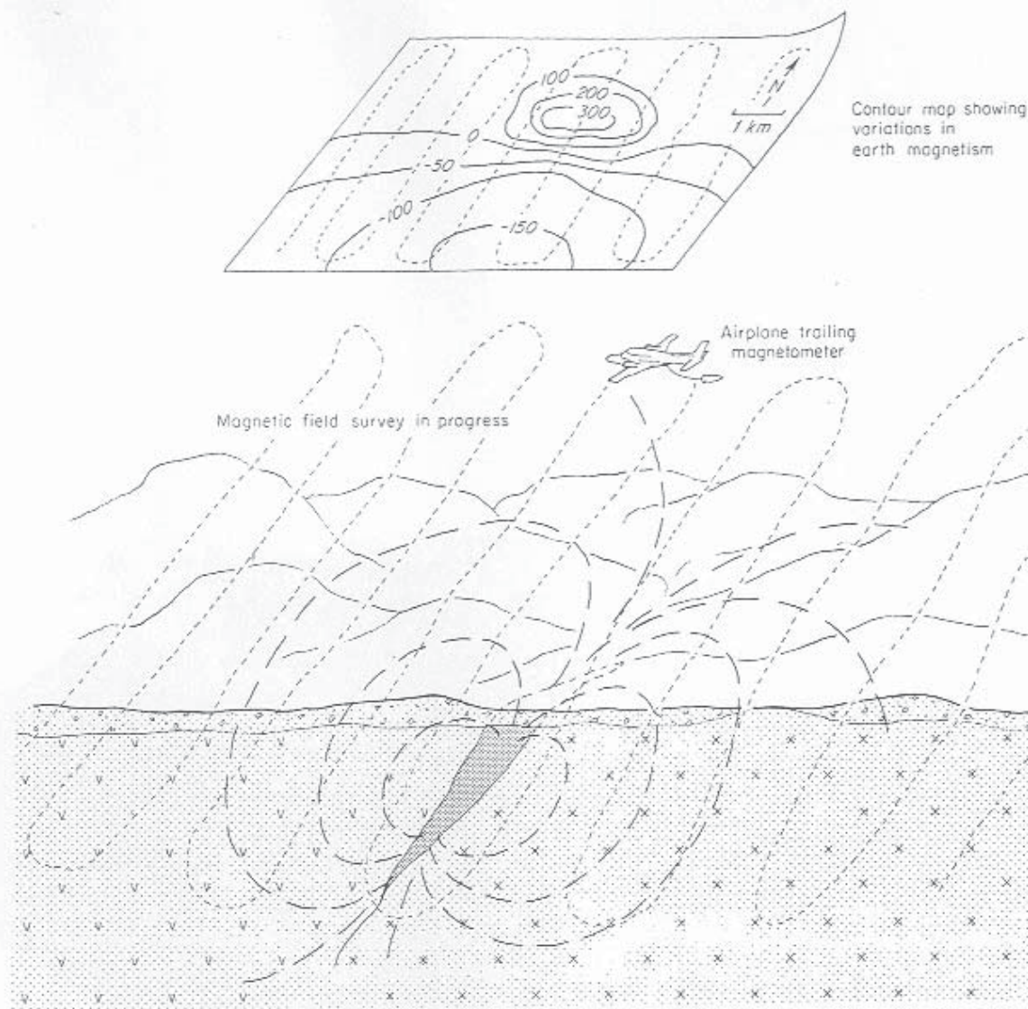
Figure 1-5 Airborne magnetometer survey for locating magnetized ores. A contour map prepared from the survey data indicates patterns of variation in
