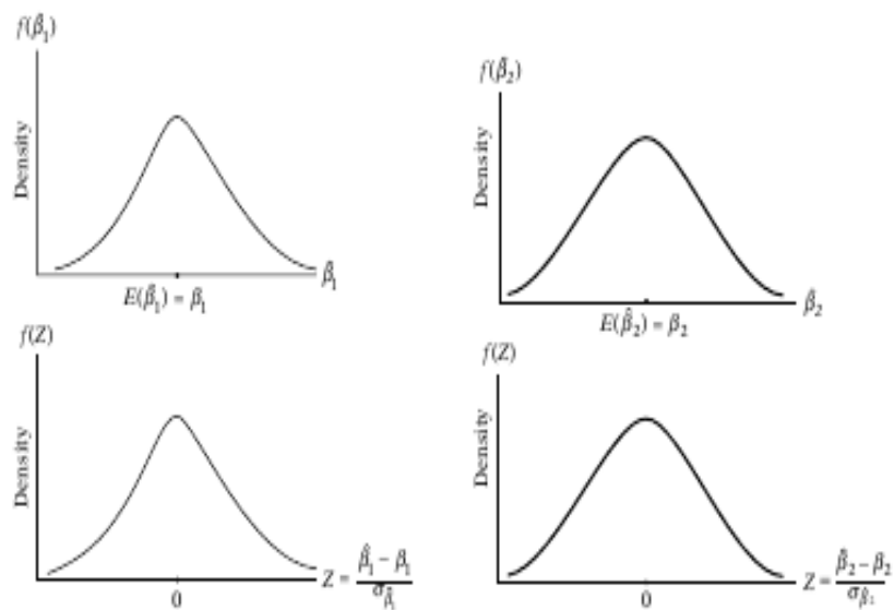
FIGURE 4.1 Probability distributions of \hat{\beta}_1 and \hat{\beta}_2 .
