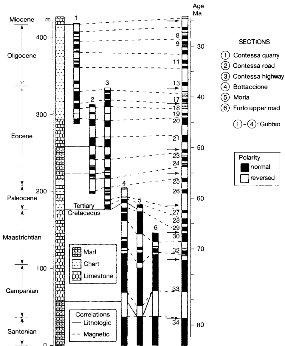
Figure 13.30 Correlation of Late Cretaceous through Cenozoic stratigraphic sections in the Umbrian Apennines on the basis of magnetostratigraphy. The sections are also correlated with the seafloor magnetic anomaly sequence (right column). Age from biostratigraphic (foraminiferal) zonation (Miocene-Santonian) is given at the left of the column showing dominant lithology. Magnetic anomaly numbers and paleontologic calibration points (shown by arrows) are noted at the left side of the seafloor polarity column. [Redrawn and modified from Lowrie, W., and W. Alvarez, 1981, One hundred million years of geomagnetic history: Geology , v. 9, Fig. 1, p. 393.]
