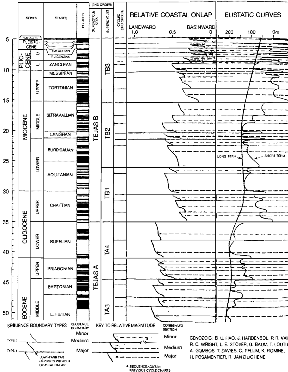
Figure 13.21 Simplified global sequence chart for part of the Tertiary and Quaternary. The polarity column shows the geomagnetic time scale (explained in Section 13.4); series and stages are discussed in Chapter 15. [After Haq, B. U., J. Hardenbol, and P. R. Vail, 1987, Chronology of fluctuating sea levels since the Triassic: Science , v. 235, Fig. 2, p. 1158. Copyright 1987 by the AAAS. As redrawn by Vail et al., 1991.]
