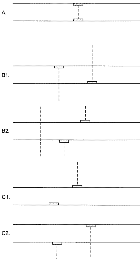
Figure 4. Examples of biostratigraphic interval zones. Vertical broken lines indicate ranges of taxa; bars indicate lowest or highest documented occurrences.
