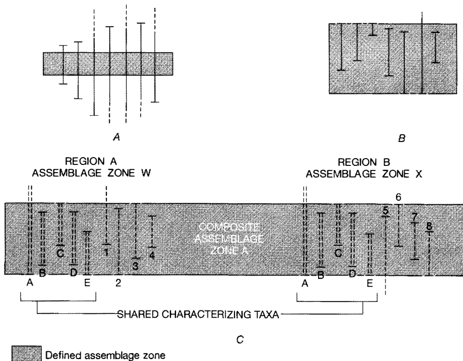
Figure 5. Examples of assemblage zone concepts.
