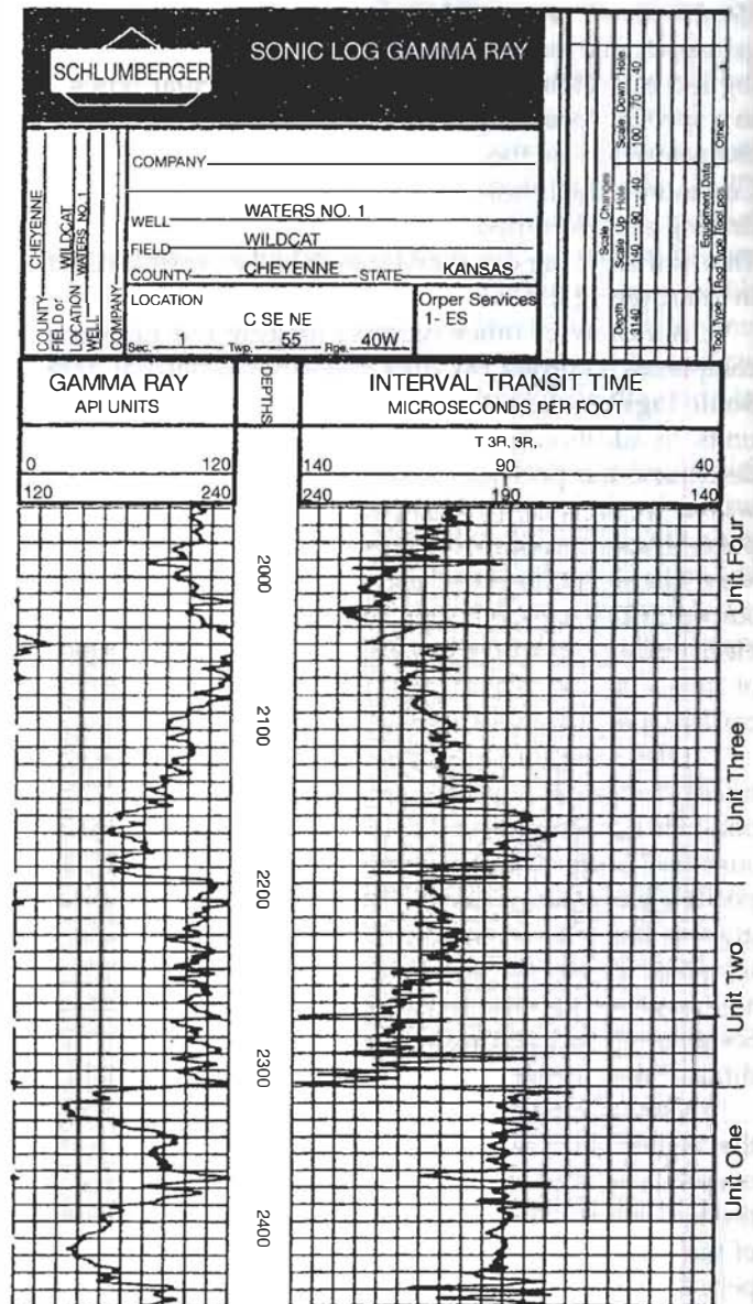
Figure 12.21 A section of a sonic-gamma ray log. The gamma ray curve is shown on the left. The sonic log (interval transit time log) is on the right. Depths (in feet) below the surface are shown in the central column. Four distinct correlatable units are indicated.
