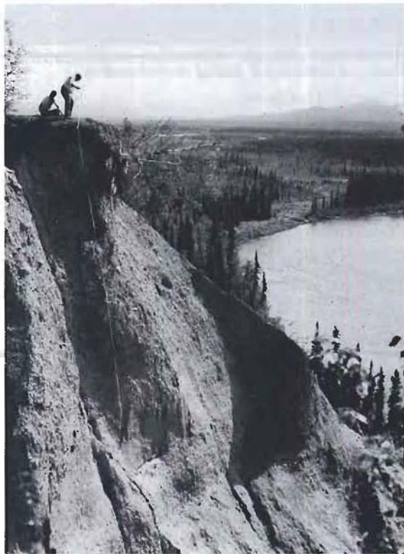
Figure 8.31 Thick, poorly stratified, poorly sorted glacial diamict (Quaternary), Alaska. [Photograph courtesy of Gail M. Ashley.]
