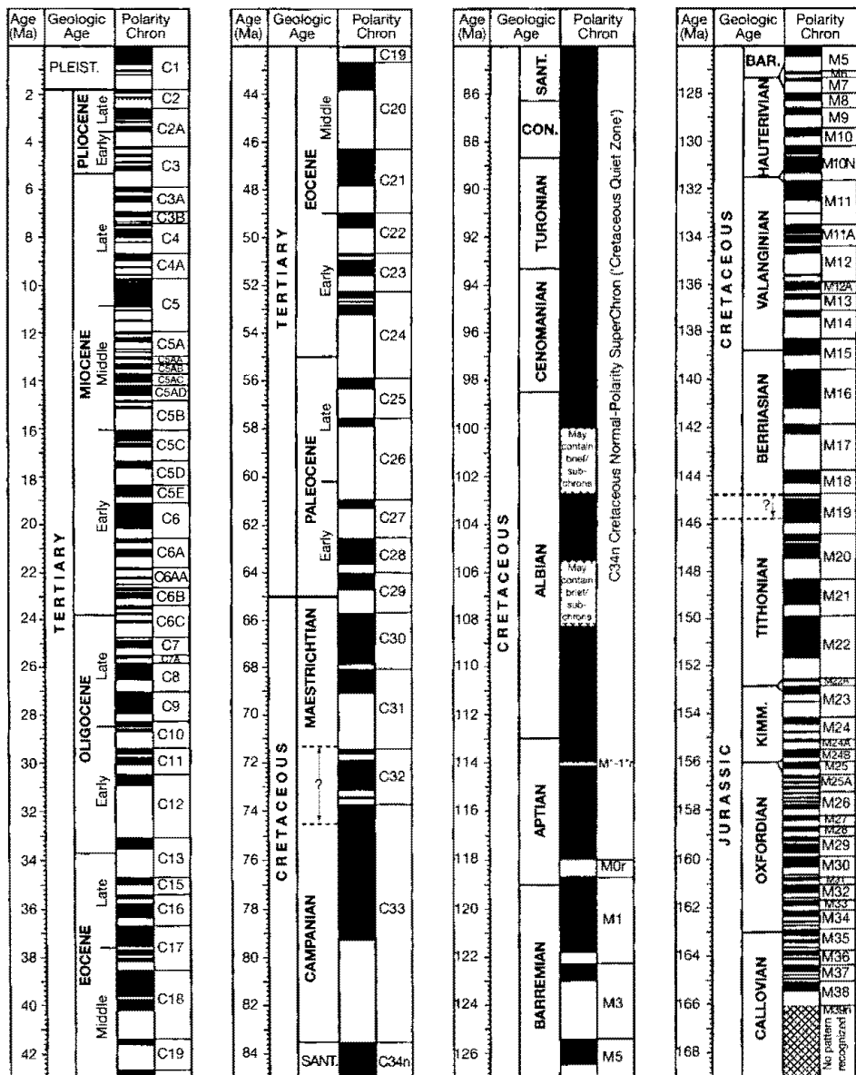
Figure 13.26 Magnetic polarity time scale for the Cenozoic-late Mesozoic. Intervals of normal polarity are shown in black, reversed polarity in white. Intervals lacking magnetostratigraphic studies or having uncertain validity are cross-hatched. [Compiled by Ogg, J. G., 1995, Magnetic polarity time scale of the Phanerozoic, in Ahrens, T. J. (ed.), Global Earth physics—A handbook of physical constants: AGU Reference Shelf 1, American Geophysical Union, Washington, D.C., Fig. 2, p. 252, reproduced by permission.]
