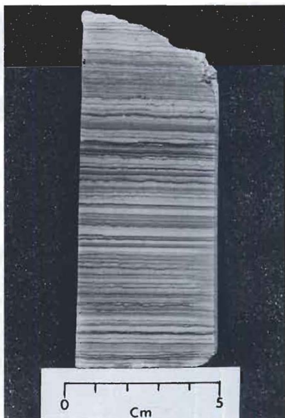
Figure 7.3 Laminated anhydrite from the Prairie Evaporite (Devonian), Canada.
