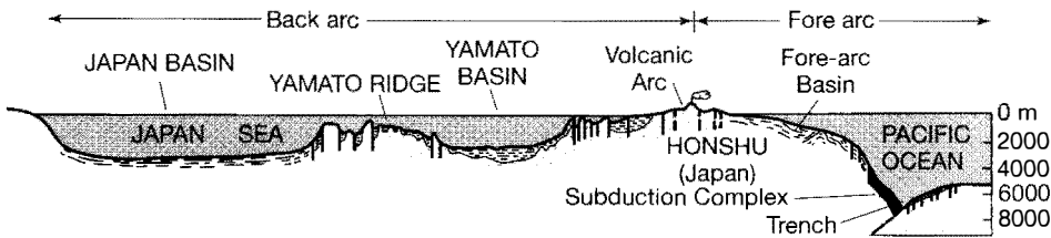
Figure 16.11 Schematic representation of an active continental margin (Japan), showing both the fore-arc and back-arc characteristics of the margin. [From Boggs, S., Jr., 1984, Quaternary sedimentation in the Japan arc-trench system: Geol. Soc. America Bull. , v. 95, Fig. 2, p. 670.]
