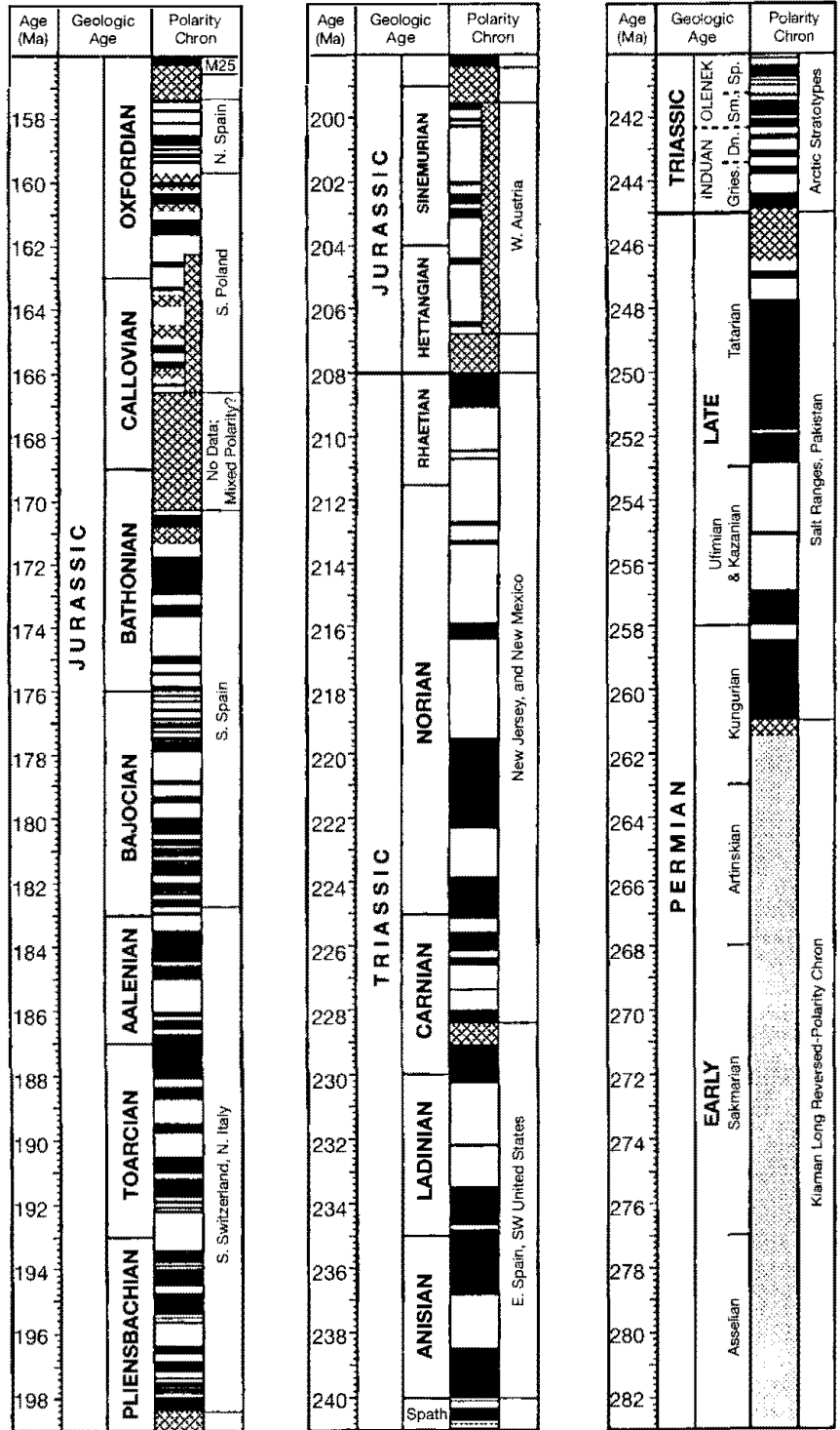
Figure 13.27 Magnetic polarity time scale for Jurassic to Permian. Intervals of normal polarity are shown in black, reversed polarity in white. Intervals lacking magnetostratigraphic studies or having uncertain validity are cross-hatched. [Compiled by Ogg, J. G., 1995, Magnetic polarity time scale of the Phanerozoic, in Ahrens, T. J. (ed.), Global Earth physics—A handbook of physical constants: AGU Reference Shelf 1 , American Geophysical Union, Washington, D.C., Fig. 3, p. 260, reproduced by permission.]
