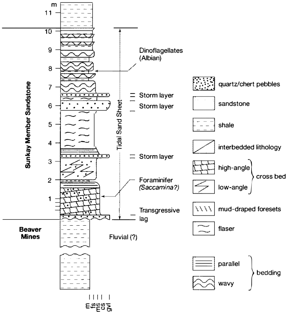
Figure 10.11 Vertical succession of sandy tidal shelf deposits in the Sunkay Sandstone Member of the Lower Cretaceous Alberta Group, southern Alberta, Canada. Symbols in the grain-size scale are gvl = gravel, cs = coarse sand, ms = medium sand, fs = fine sand, and m = mud (silt-clay). [After Banerjee, I., 1991, Tidal sand sheets of the late Albian Joli Fou-Kiowa-Skull Creek marine transgression, Western Interior Seaway of North America in Smith, R. G., et al. (eds.), Clastic tidal sedimentology: Canadian Soc. Petroleum Geologists Mem. 16 , Fig. 9, p. 334.]
