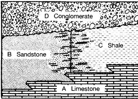
A.-- Boundaries at sharp lithologic contacts and in a laterally gradational sequence.
