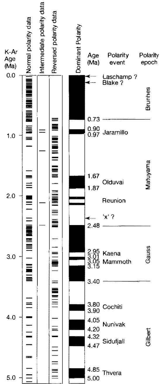
Figure 13.24 Late Cenozoic (Pliocene-Pleistocene) geomagnetic polarity time scale. Each horizontal line in the columns labeled normal polarity, intermediate polarity, or reversed polarity represents an igneous rock for which both K-Ar age and geomagnetic polarity have been determined. Auxiliary information from marine magnetic anomaly profiles and deep-sea core paleomagnetism have also been used. Black pattern in the dominant-polarity column indicates normal polarity; white indicates reversed polarity. Arrows indicate disputed short polarity intervals or geomagnetic "excursions"; numbers to the right of the polarity column indicate interpreted ages of polarity boundaries. [After Maniken, E. A., and G. B. Dalrymple, 1979, Revised geomagnetic polarity time scale for the interval 0–5 m.y. B. P.: Jour. Geophysical Research, v. 84, Fig. 3, p. 624.]
