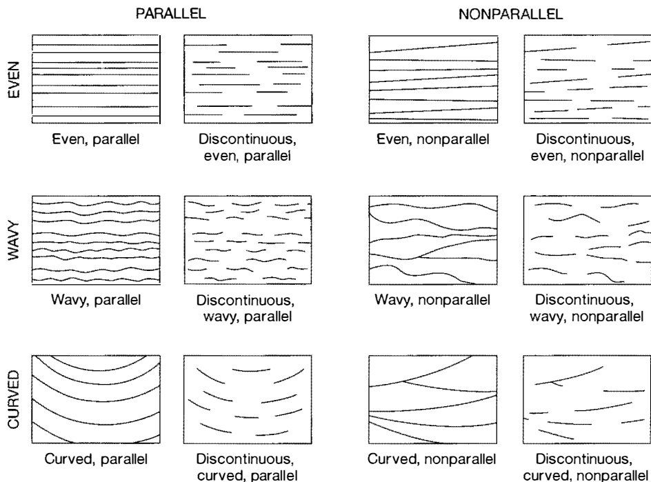
Figure 4.3 Descriptive terms used for the configuration of bedding surfaces. [From Campbell, C. V., 1967, Lamina, laminaset, bed and bedset : Sedimentology, v. 8, Fig. 2, p. 18, reprinted by permission of Elsevier Science Publishers, Amsterdam.]
