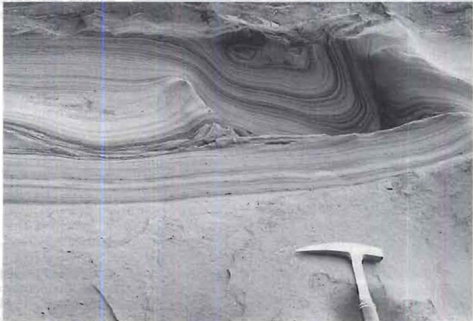
Figure 4.26 Convolute lamination in fine-grained sandstone and shale, Coaledo Formation (Eocene), southwestern Oregon. Note absence of deformation in the underlying layers.
