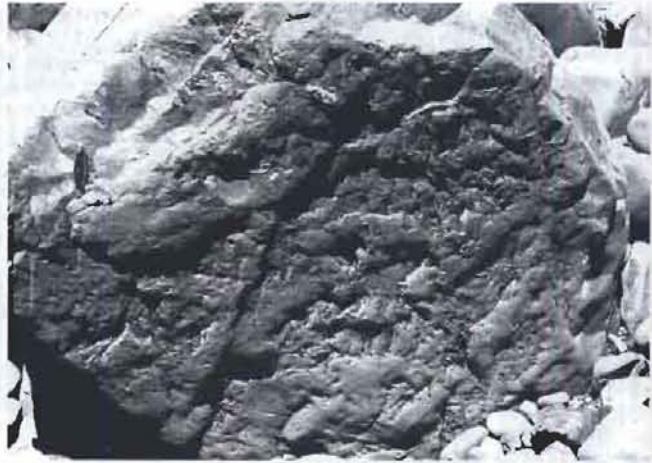
Figure 4.37 Irregularly shaped load casts on the base of a loose slab of Cretaceous sandstone, southern Oregon coast.
