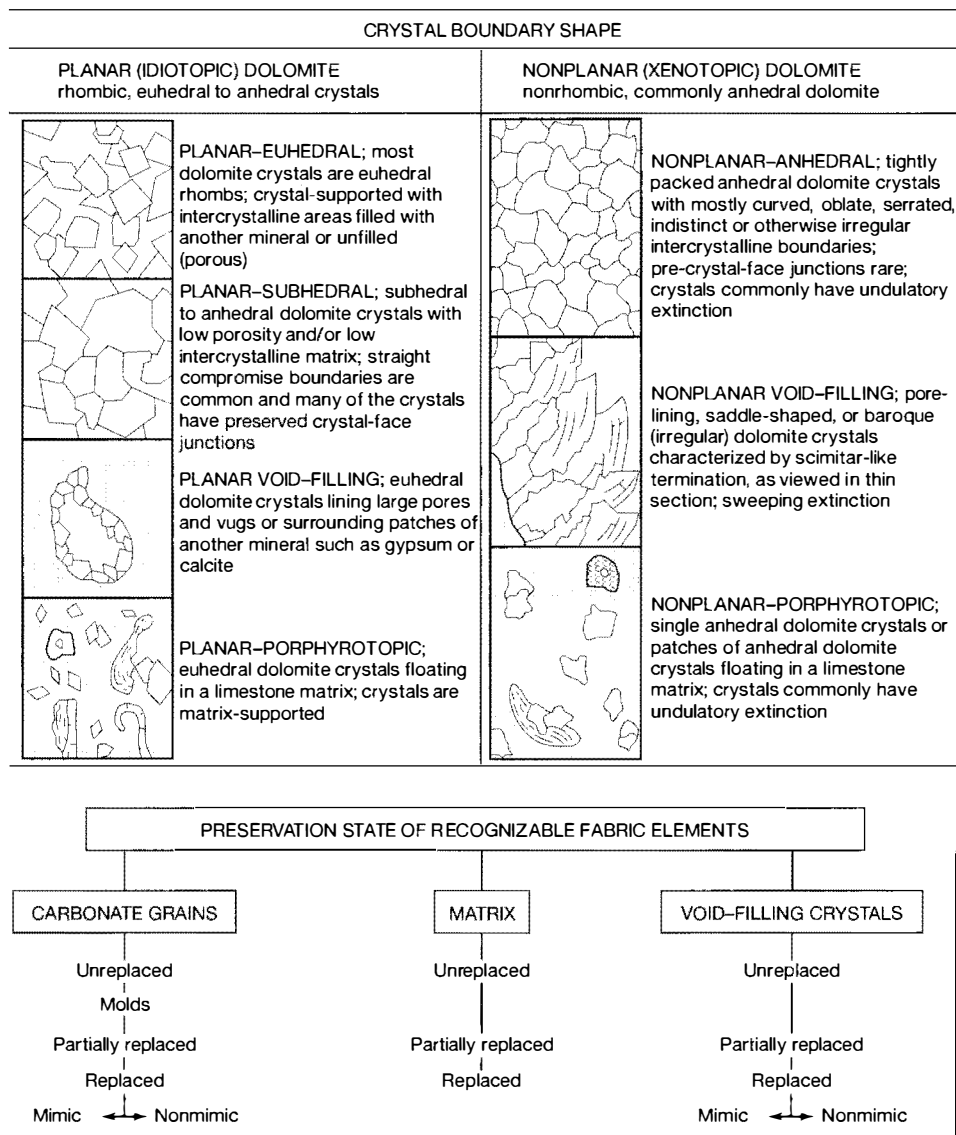
Figure 6.6 Classification of dolomite textures. [After Gregg, J. M., and D. F. Sibley, 1984, Epigenetic dolomitization and the origin of xenotopic dolomite texture: Jour. Sed. Petrology , v. 54, Fig. 6, p. 913, and Sibley, D. F., and Gregg, J. M., 1987, Classification of dolomite rock textures: Jour. Sed. Petrology , v. 57, Fig. 1, p. 968; figures reprinted by permission of Society of Economic Paleontologists and Mineralogists, Tulsa, Okla.]
