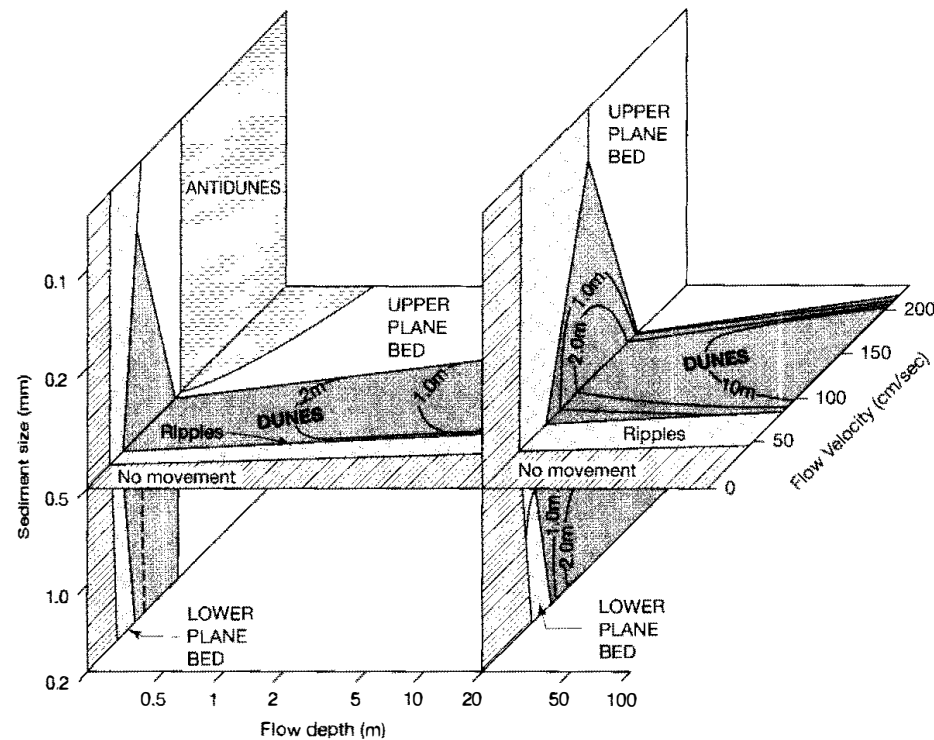
Figure 4.11 Generalized three-dimensional depth-velocity-grain-size diagram showing the relationship among bed phases and grain size for a wide variety of flow velocities and flow depths. Diagram based on both flume data and observations of natural flows. [After Rubin, M. D., and D. S. McCulloch, 1980, Single and superimposed bedforms: A synthesis of San Francisco Bay and fluvial observations: Sed. Geology , v. 26, Fig. 11, p. 224, reprinted by permission of Elsevier Science Publishers, Amsterdam.]
