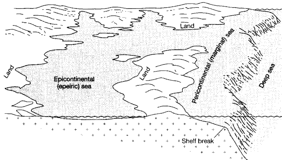
Figure 10.2 Schematic diagram illustrating the difference between pericontinental (continental shelf) and epicontinental shallow-marine environments. [After Heckel, P. H., 1972, Reconigition of ancient shallow marine environments , in Rigby, J. K., and W. K. Hamblin (eds.), Recognition of ancient sedimentary environments: SEPM (Society for Sedimentary Geology) Spec. Pub. 16, Fig. 1, p. 227, reprinted by permission. ]
