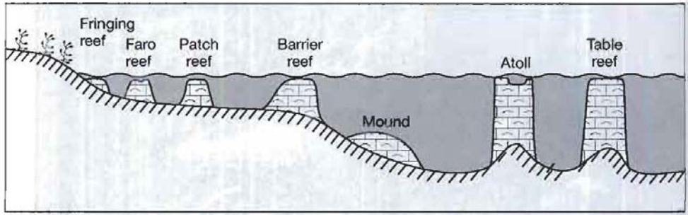
Figure 11.14 Schematic representation of the principal kinds of reefs. Based on Tucker, M. E., and V. P. Wright, 1990, Carbonate sedimentology: Blackwell Scientific Publications, Fig. 4.86, p. 192.
