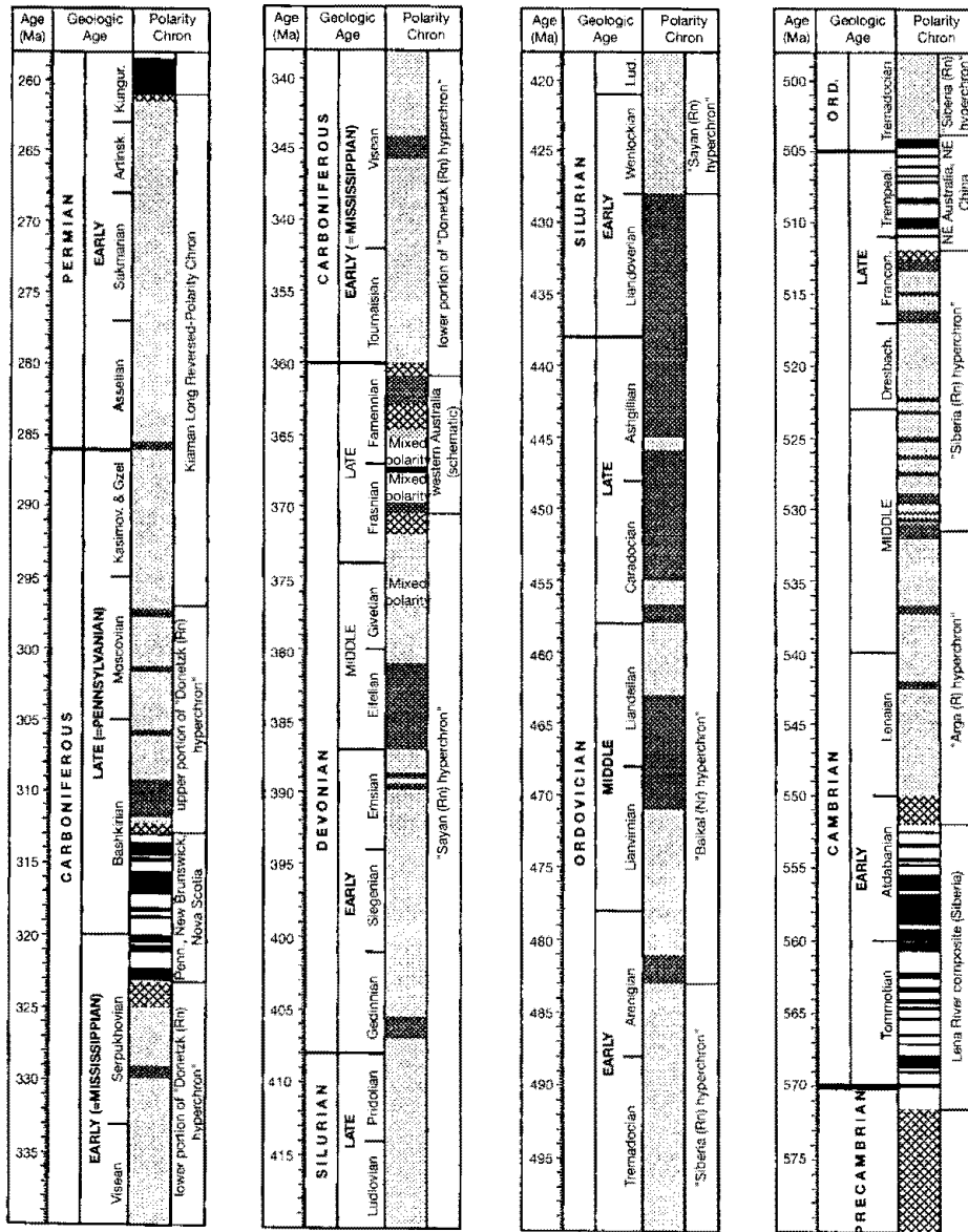
Figure 13.28 Magnetic polarity time scale for the Paleozoic. Intervals of normal polarity are shown in black, reversed polarity in white. Intervals lacking magnetostratigraphic studies or having uncertain validity are cross-hatched. Unverified Paleozoic polarity intervals from the Soviet scale (Khramov and Rodionov, 1981) are shown as shades of gray. [Compiled by Ogg, J.G., 1995, Magnetic polarity time scale of the Phanerozoic, in Ahrens, T. J. (ed.), Global Earth physics—A handbook of physical constants: AGU Reference Shelf 1, American Geophysical Union, Washington, D.C., Fig. 4, p. 265, reproduced by permission.]
