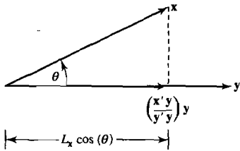
Figure 2.5 The projection of \mathbf{x} on \mathbf{y} .
