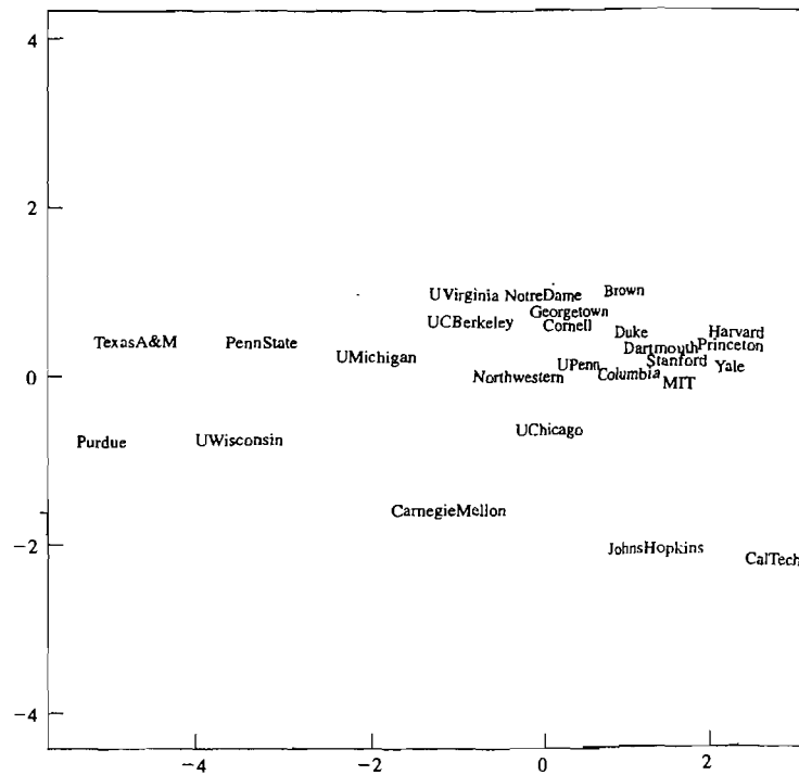
Figure 12.19 A two-dimensional representation of universities produced by metric multidimensional scaling.
