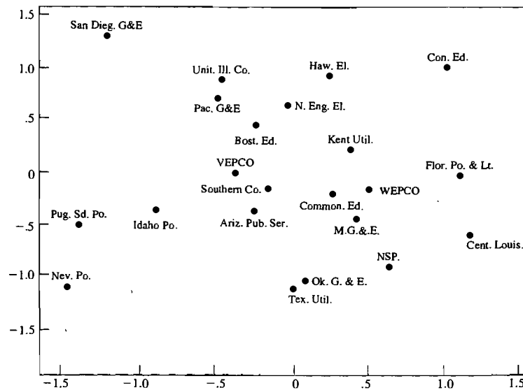
Figure 12.18 A geometrical representation of utilities produced by multidimensional scaling.
