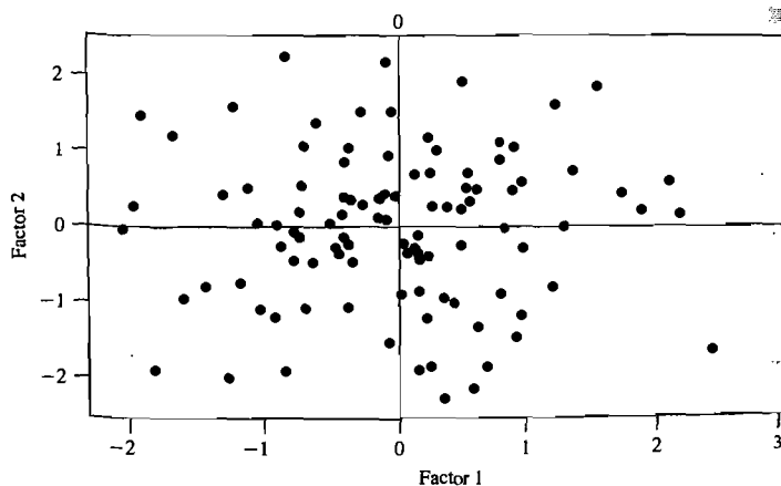
Figure 9.4 Factor scores using (9-58) for factors 1 and 2 of the stock-price data (maximum likelihood estimates of the factor loadings).
