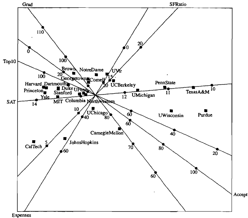
Figure 12.25 An alternative biplot of the data on universities.
