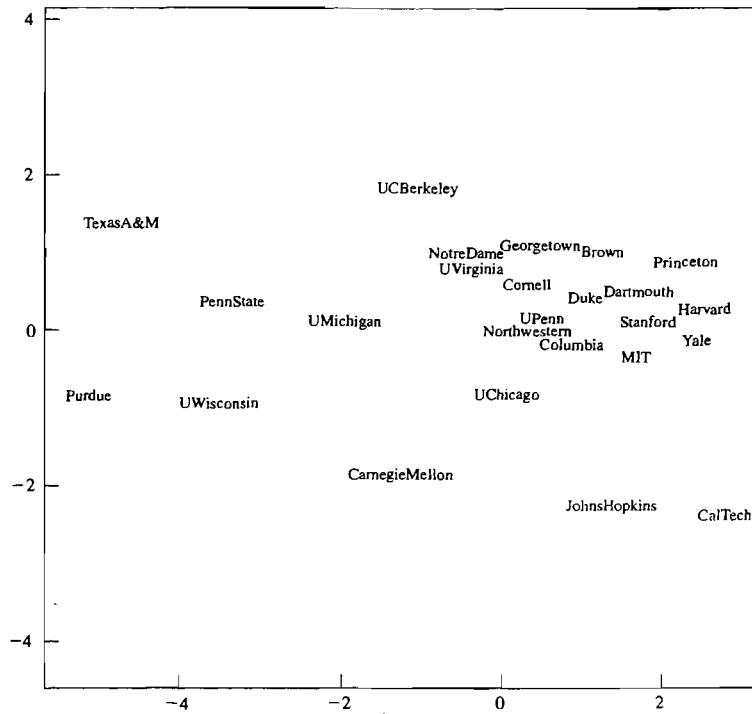
Figure 12.20 A two-dimensional representation of universities produced by nonmetric multidimensional scaling.
