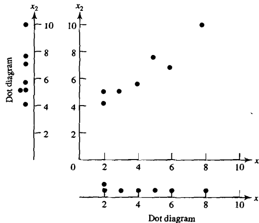
Figure 1.1 A scatter plot and marginal dot diagrams.
