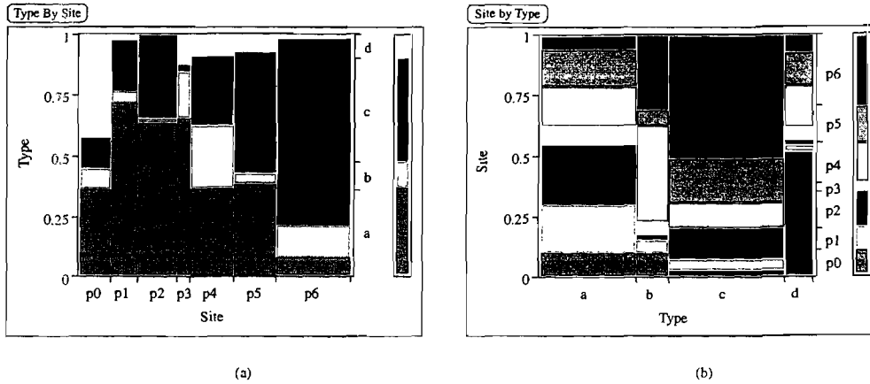
Figure 12.21 Site and pottery type profiles for the data in Table 12.8.
