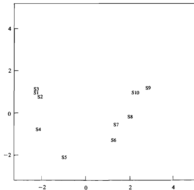
Figure 12.26 Metric multidimensional scaling of the data on forests.
