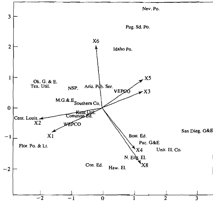
Figure 12.23 A biplot of the data on public utilities.
