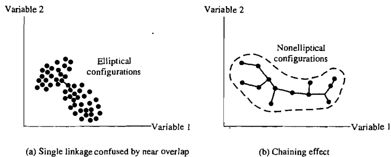
Figure 12.5 Single linkage clusters.
