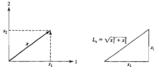
Figure 2.3 Length of \mathbf{x} = \sqrt{x_1^2 + x_2^2} .
