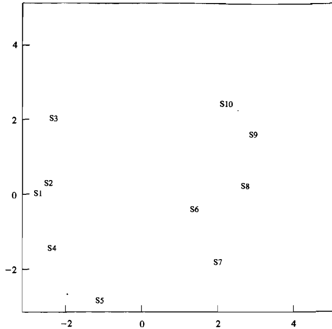
Figure 12.27 Nonmetric multidimensional scaling of the data on forests.
