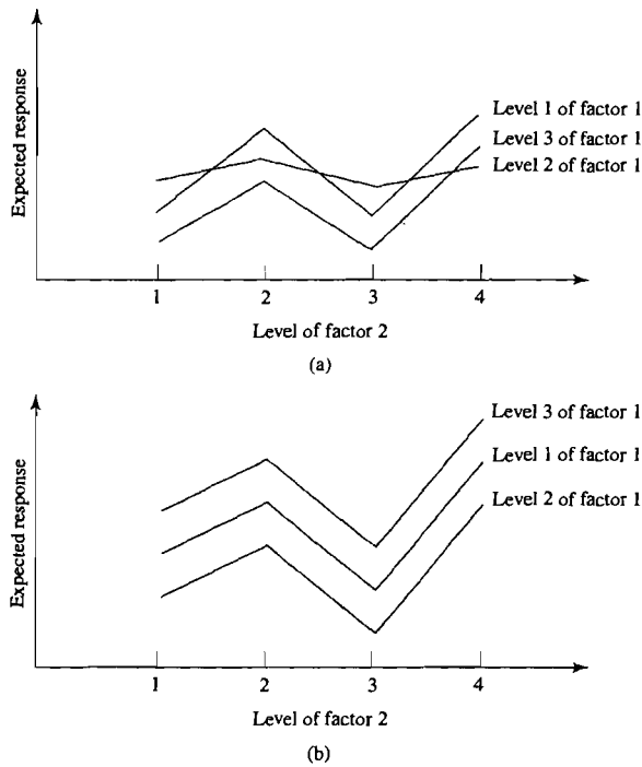
Figure 6.3 Curves for expected responses (a) with interaction and (b) without interaction.
