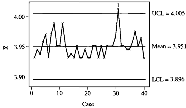
Figure 5.11 The univariate \bar{X} -chart for \ln(\text{gas flow}) .
