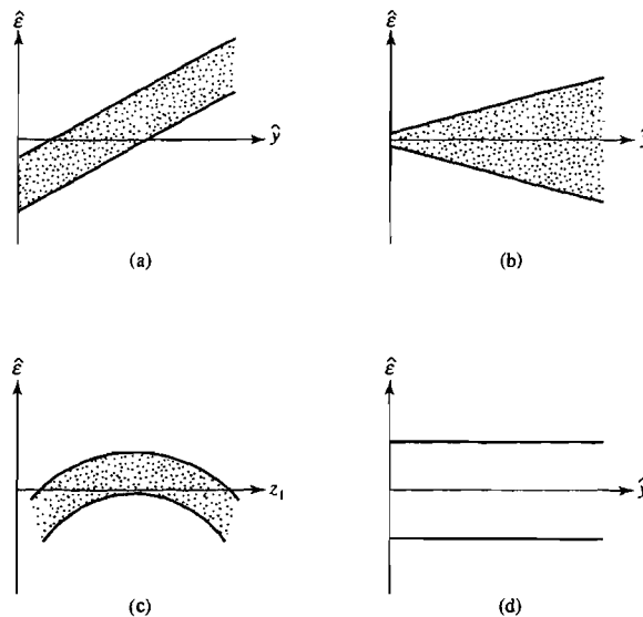
Figure 7.2 Residual plots.
