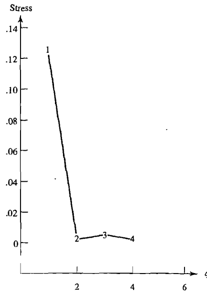
Figure 12.16 Stress function for airline distances between cities.
