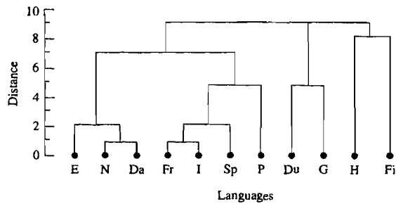
Figure 12.4 Single linkage dendrograms for distances between numbers in 11 languages.
