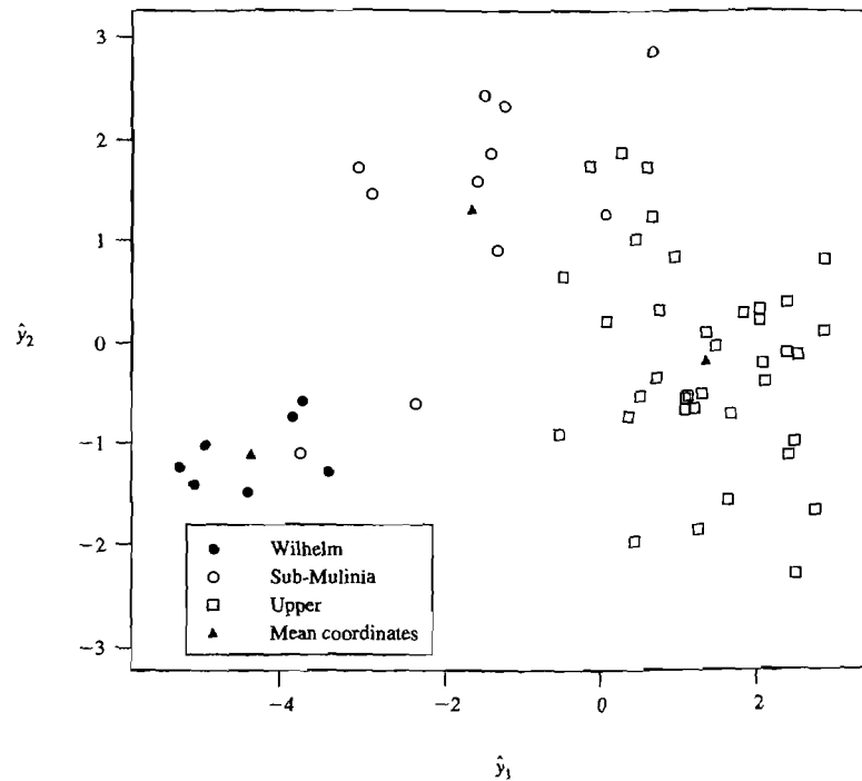
Figure 11.12 Crude-oil samples in discriminant space.
