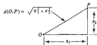
Figure 1.19 Distance given by the Pythagorean theorem.
