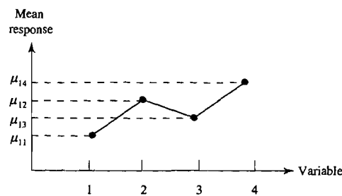
Figure 6.4 The population profile p = 4 .
