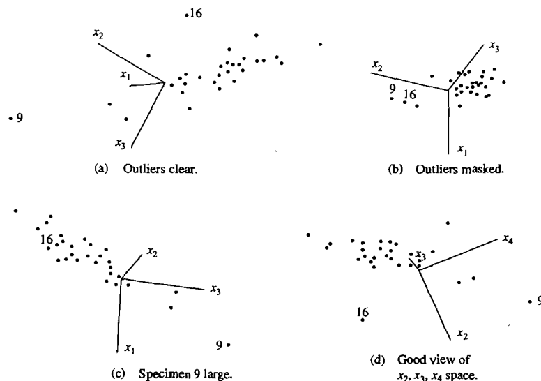
Figure 1.12 Three-dimensional perspectives for the lumber stiffness data.
