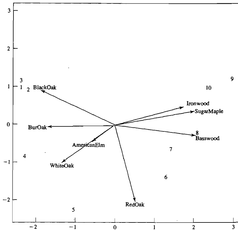
Figure 12.29 The biplot of the data on forests.
