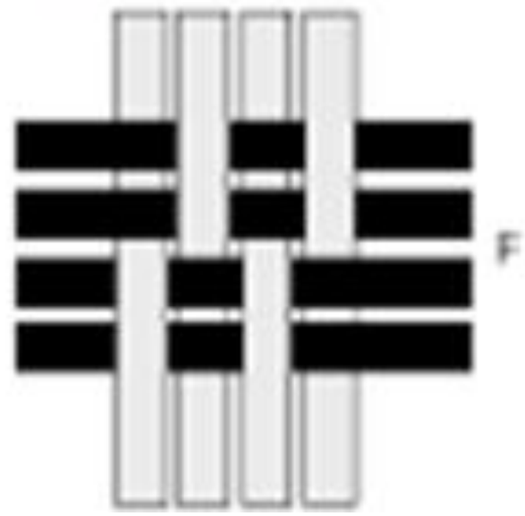
Warp rib Weave-regular
