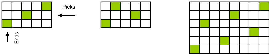
Reverse Sateen or Strip Sateen
