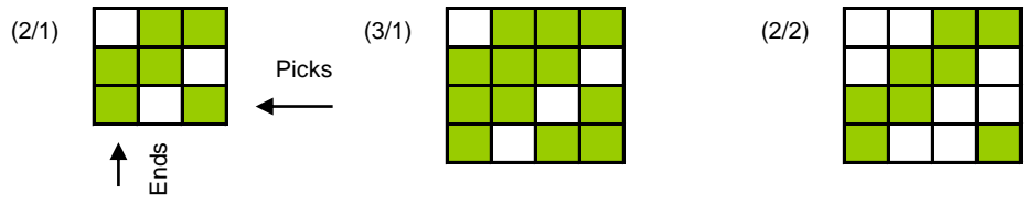
Broken Twill
