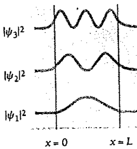
Figure 5.8 Wave functions and probability densities of a particle in a finite potential well. The particle has a certain probability of being found outside the wall.
