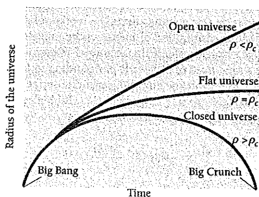
Figure 13.13 Three cosmological models that follow from the equations of general relativity. The quantity \rho is the average density of the universe and \rho_c , the critical density, is in the neighborhood of 9 \times 10^{-27} \text{ kg/m}^3 , equivalent to about 5 hydrogen atoms per cubic meter.
