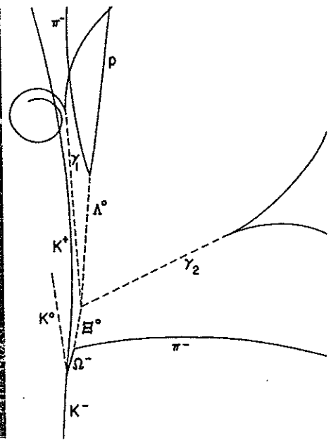
Liquid hydrogen bubble chamber photograph showing the production of a \Omega^- baryon by the interaction of a K^- meson (moving upward from the bottom) with a proton together with the subsequent decay of the \Omega^- into a \Xi^0 baryon and a \pi^- meson. The sketch shows the identities of the charged particles that caused each track; the dashed lines indicate the paths of neutral particles that leave no tracks. A magnetic field deflected the paths of the charged particles and enabled their momenta to be determined. The \Omega^- baryon was predicted theoretically before its discovery in 1964. (Courtesy Brookhaven National Laboratory)
