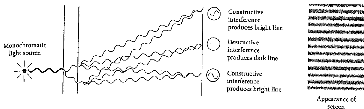
Figure 2.4 Origin of the interference pattern in Young's experiment. Constructive interference occurs where the difference in path lengths from the slits to the screen is \theta , \lambda , 2\lambda , . . . . Destructive interference occurs where the path difference is \lambda/2 , 3\lambda/2 , 5\lambda/2 , . . . .
