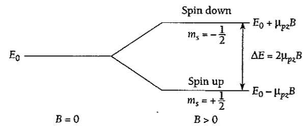
Figure 11.5 The energy levels of a proton in a magnetic field are split into spin-up ( S_z parallel to B ) and spin-down ( S_z antiparallel to B ) sublevels.
