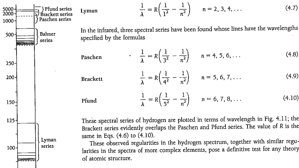
Figure 4.11 The spectral series of hydrogen. The wavelengths in each series are related by simple formulas.
