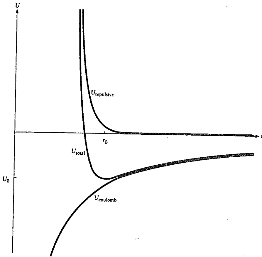
Figure 10.7 How the ionic potential energies in an ionic crystal vary with ionic separation r . The minimum value U_0 of U_{\text{total}} occurs at an equilibrium separation of r_0 .
