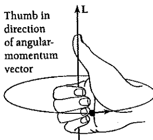
Figure 6.3 The right-hand rule for angular momentum.
