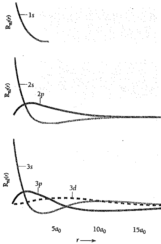
Figure 6.8 The variation with distance from the nucleus of the radial part of the electron wave function in hydrogen for various quantum states. The quantity a_0 = 4\pi\epsilon_0\hbar^2/me^2 = 0.053 \text{ nm} is the radius of the first Bohr orbit.
