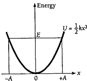
Figure 5.10 The potential energy of a harmonic oscillator is proportional to x^2 , where x is the displacement from the equilibrium position. The amplitude A of the motion is determined by the total energy E of the oscillator, which classically can have any value.
