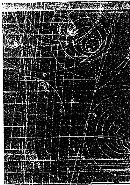
Liquid hydrogen bubble chamber photograph showing the production of a \Omega^- baryon by the interaction of a K^- meson (moving upward from the bottom) with a proton together with the subsequent decay of the \Omega^- into a \Xi^0 baryon and a \pi^- meson. The sketch shows the identities of the charged particles that caused each track; the dashed lines indicate the paths of neutral particles that leave no tracks. A magnetic field deflected the paths of the charged particles and enabled their momenta to be determined. The \Omega^- baryon was predicted theoretically before its discovery in 1964. (Courtesy Brookhaven National Laboratory)
