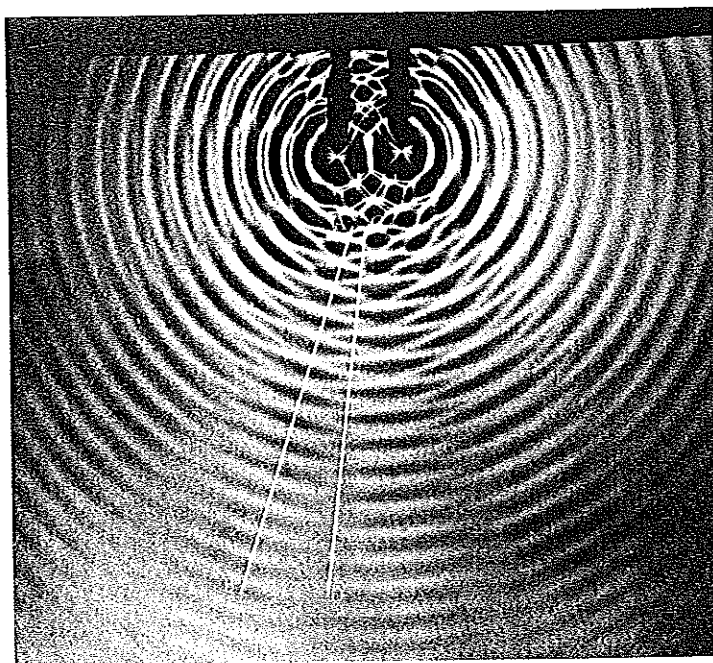
The interference of water waves. Constructive interference occurs along the line AB and destructive interference occurs along the line CD.
