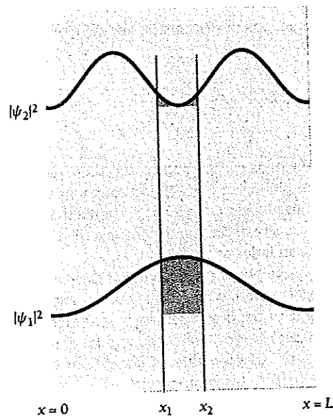
Figure 5.6 The probability P_{x_1, x_2} of finding a particle in the box of Fig. 5.5 between x_1 = 0.45L and x_2 = 0.55L is equal to the area under the |\psi|^2 curves between these limits.
