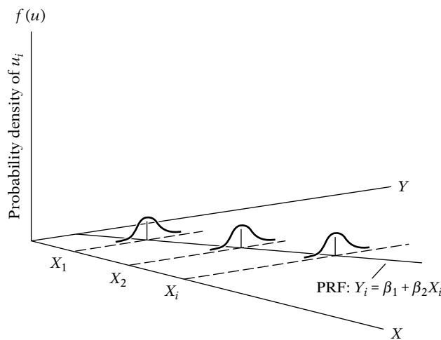
FIGURE 3.4 Homoscedasticity.
