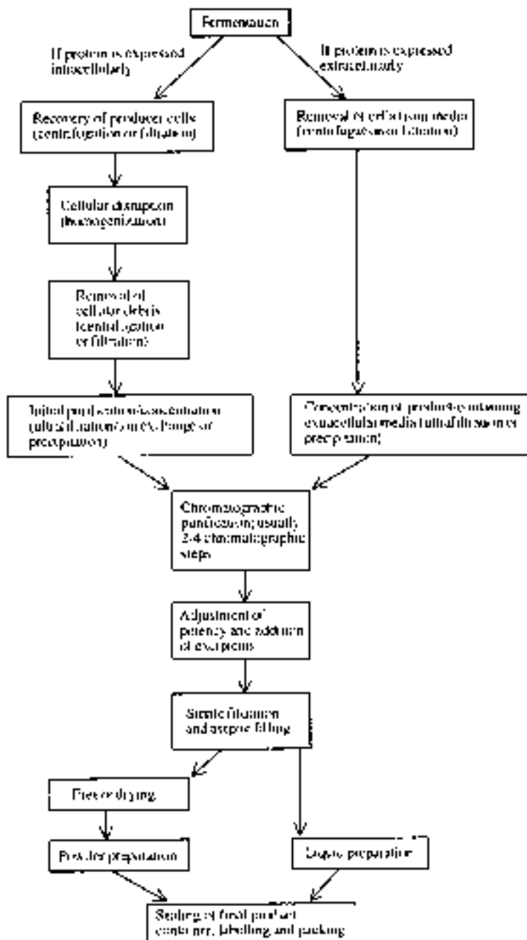
Figure 3.16. Overview of a generalized downstream processing procedure employed to produce a finished product (protein) biopharmaceutical. Quality control also plays a prominent role in downstream processing. QC personnel collect product samples during/after each stage of processing. These samples are analysed to ensure that various in-process specifications are met. In this way, the production process is tightly controlled at each stage
