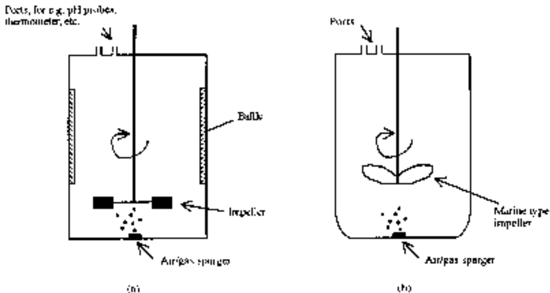
Figure 3.15. Design of a generalized microbial cell fermentation vessel (a) and an animal cell bioreactor (b). Animal cell bioreactors display several structural differences as compared to microbial fermentation vessels. Note in particular (i) the use of a marine-type impeller (some animal cell bioreactors—air lift fermenters—are devoid of impellers, and use sparging of air-gas as the only means of media agitation); (ii) the absence of baffles and; (iii) curved internal surfaces at the bioreactor base. These modifications aim to minimize damage to the fragile animal cells during culture. Note that various additional bioreactor configurations are also commercially available. Reprinted by permission of John Wiley & Sons Ltd from Walsh (2002)
