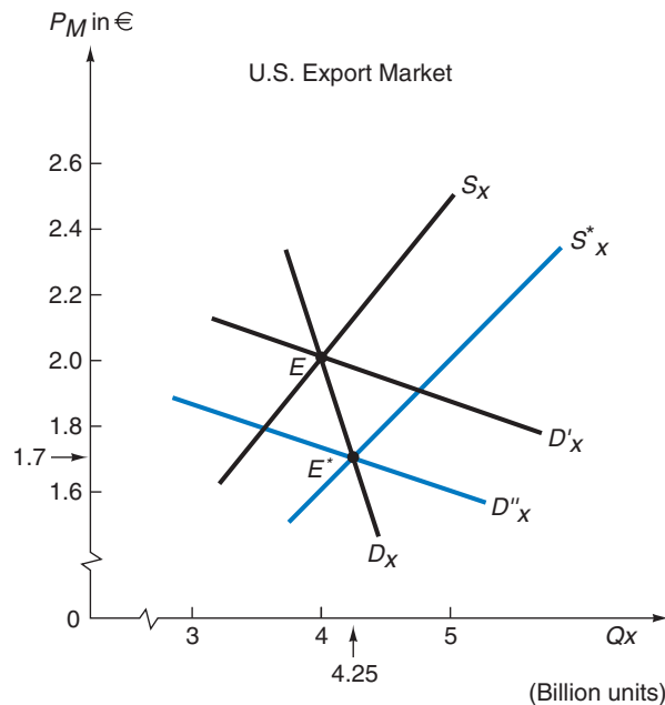
FIGURE 16.4. The Identification Problem.
