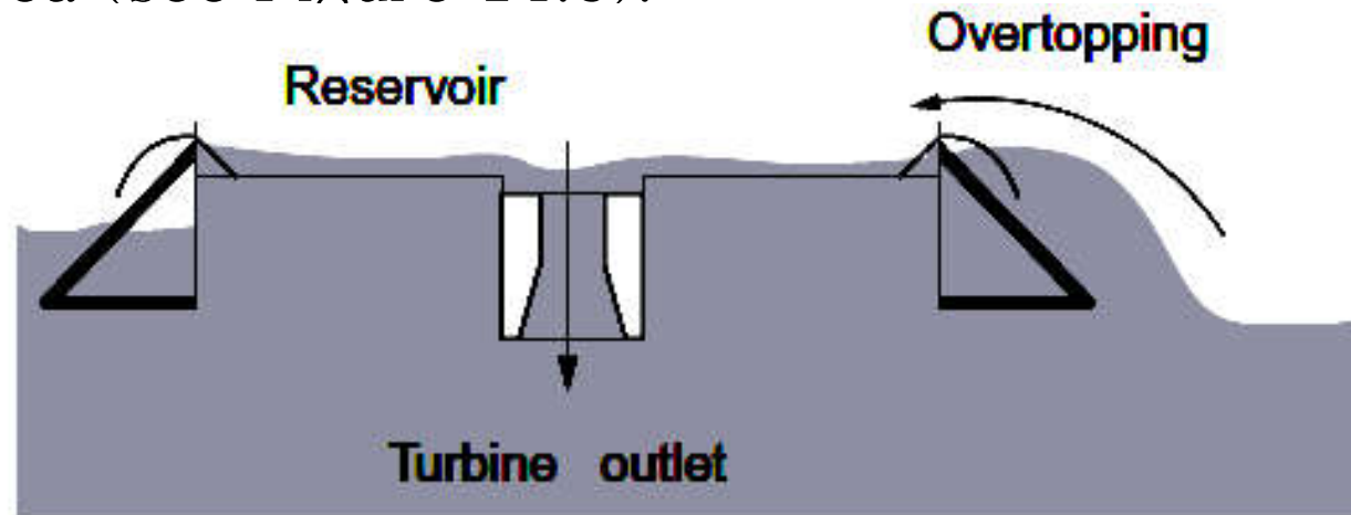
FIGURE 14.5 Schematic view of an overtopping wave energy device. Eric Fr  s-Madsen.
