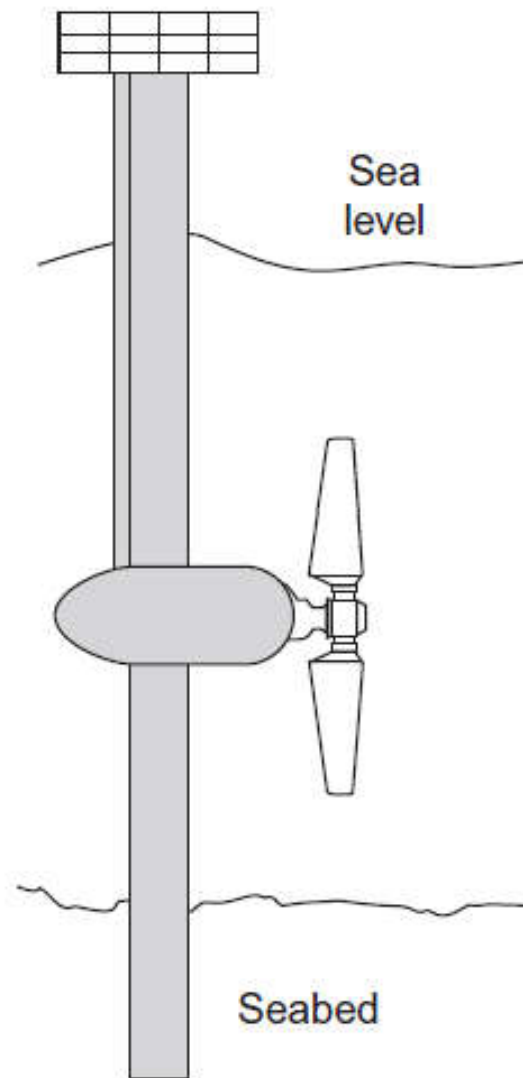
FIGURE 14.9 Schematic of a horizontal axis turbine, marine current converter.
