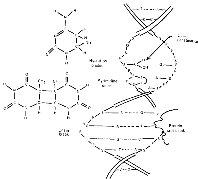
Figure 9.1 Mutagenic photochemical reactions in DNA helix, 5-hydro-6-hydroxy cytosine and thymine dimer.
