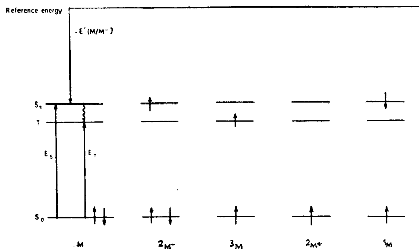
Figure 4.13 Electron configuration of dyes in ground excited singlet and triplet states and in oxidized and reduced forms: (M) ground singlet, ( M^- ) reduced form, ( M ) triplet state, ( M^+ ) oxidized form and ( 1M ) excited singlet state.
