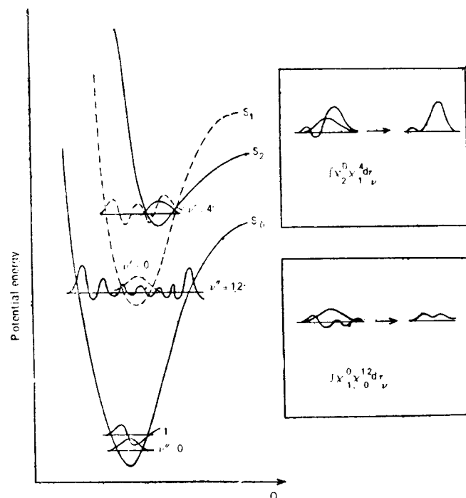
Figure 5.2 Potential energy surface for S_0 , S_1 and S_2 and Franck-Condon overlap integral. Inset: (A) Overlap integral between S_0^{v''=12} and S_1^{v'=0} and (B) S_1^{v'=4} and S_2^{v''=0} states for horizontal transfer of energy.
