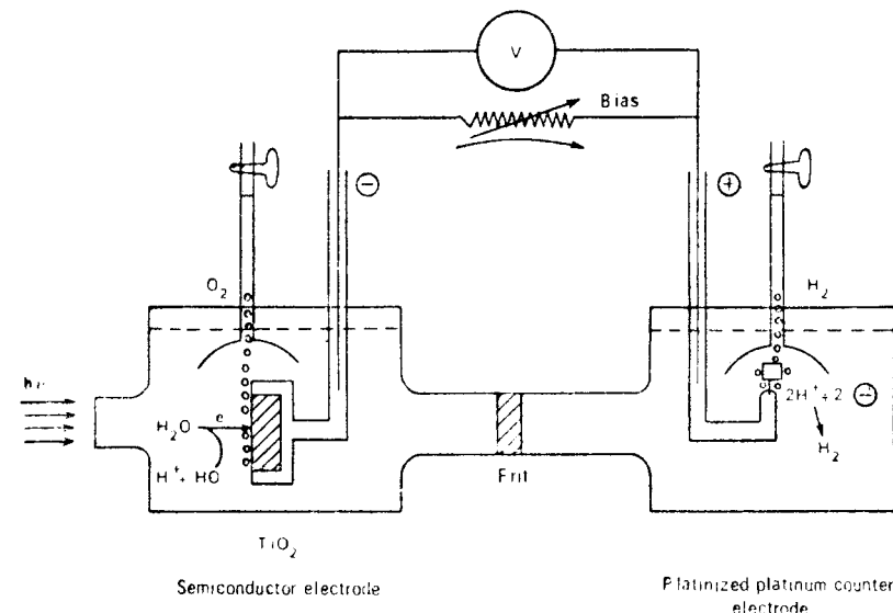
Figure 9.9 Honda's cell for photolysis of water on \text{TiO}_2 electrode.
