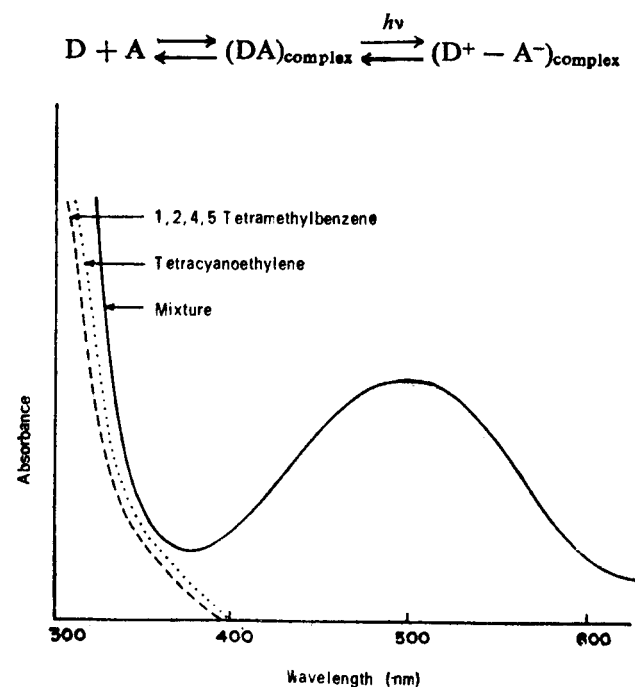
Figure 3.16 Charge transfer band for the complex between 1, 2, 4, 5-tetramethylbenzene and tetracyanoethylene. [Adapted from Britain, Gerge and Wells, Introduction to Molecular Spectroscopy-Theory and Experiment . Academic Press, 1972.]
