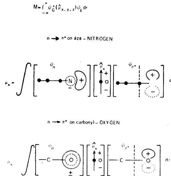
Figure 3.9 Schematic representation of transition moment integral in pyridine and formaldehyde. (Ref. 3.4).
