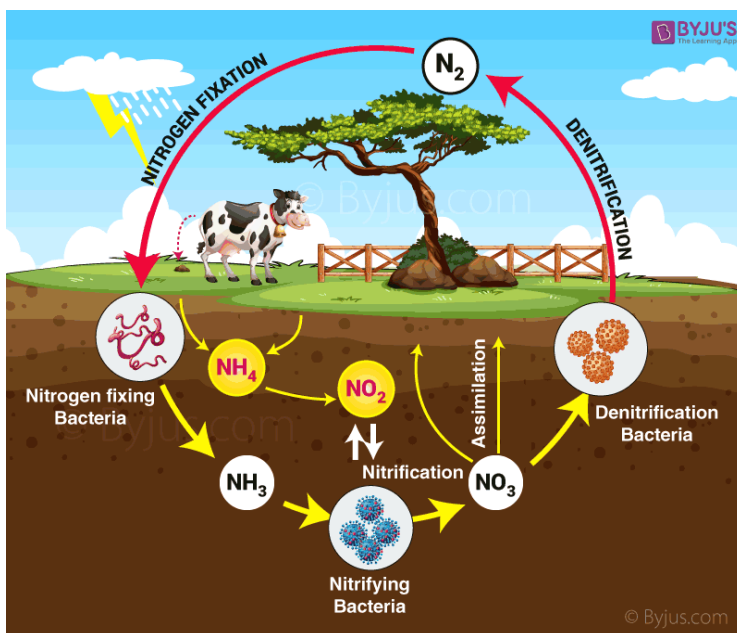
Nitrogen cycle diagram
