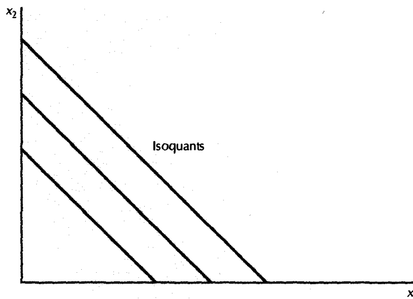
Perfect substitutes. Isoquants for the case of perfect substitutes.
