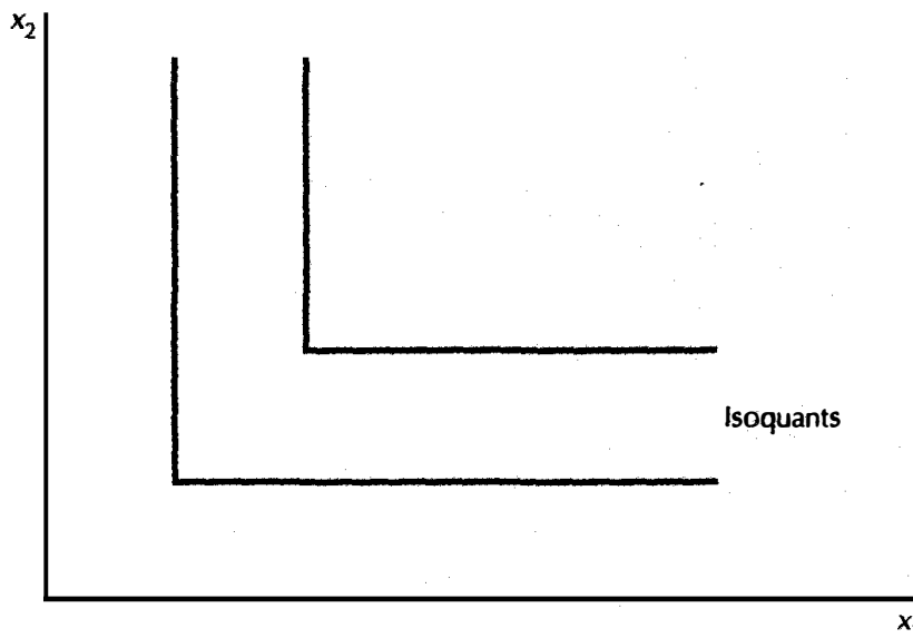
Fixed proportions. Isoquants for the case of fixed proportions.
