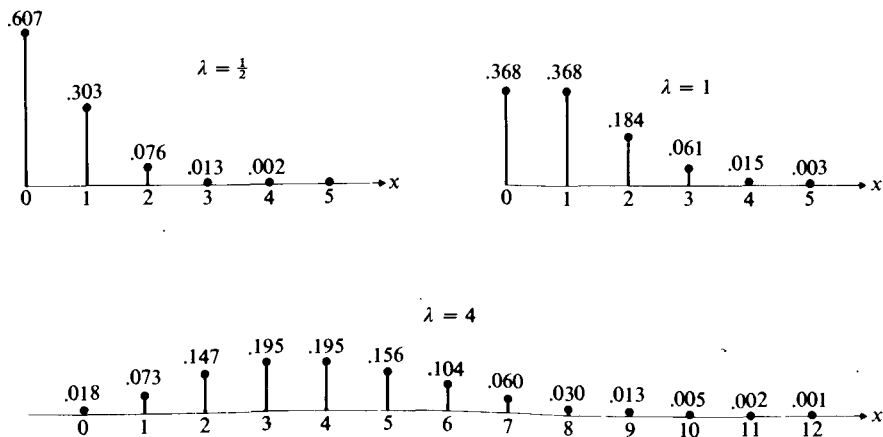
FIGURE 5 Poisson densities.
