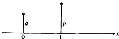
FIGURE 2 Bernoulli density.
