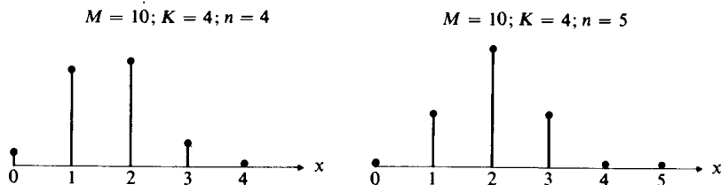
FIGURE 4 Hypergeometric densities.
