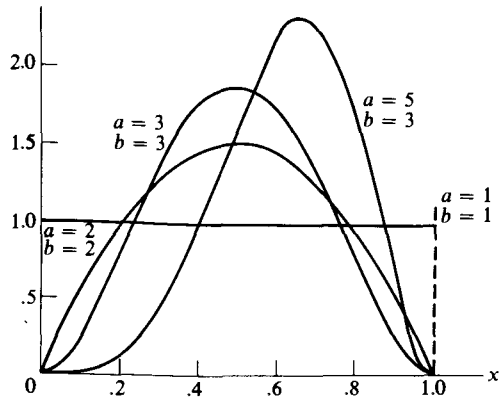
FIGURE 12 Beta densities.
