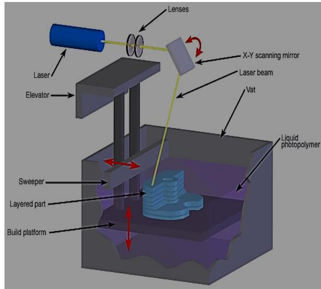
(a) Stereo lithography (SLA) working
