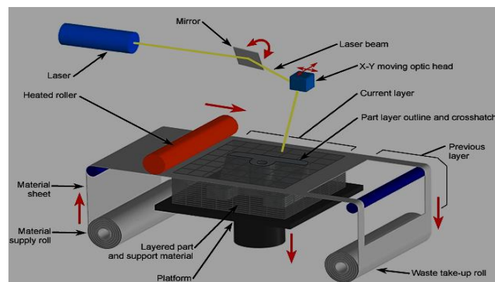
(a) Laminated Object Manufacturing (LOM)
