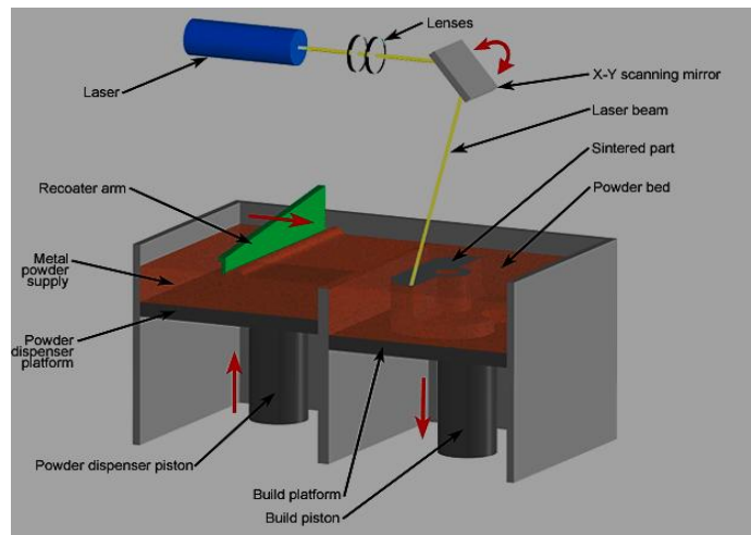
(a) Direct Metal Laser Sintering (DMLS)
