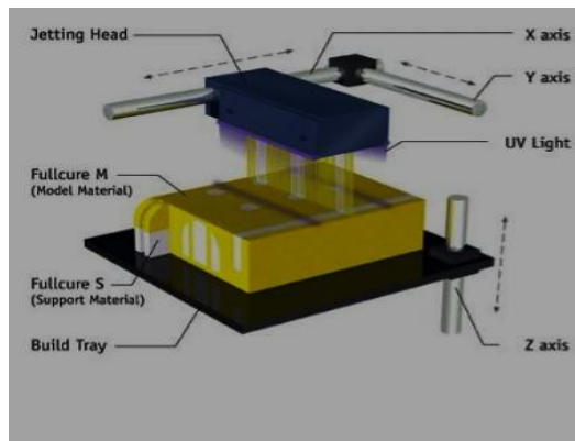
(a) Poly-jet Photopolymer
