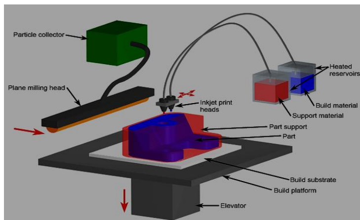
(a) Inkjet Printing
