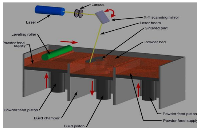
(a) Selective Laser Sintering (SLS)
