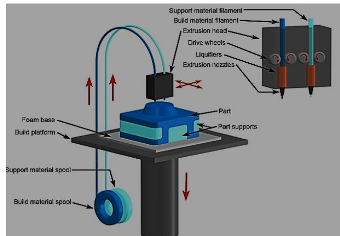
(a) Fused Deposition Modeling (FDM)
