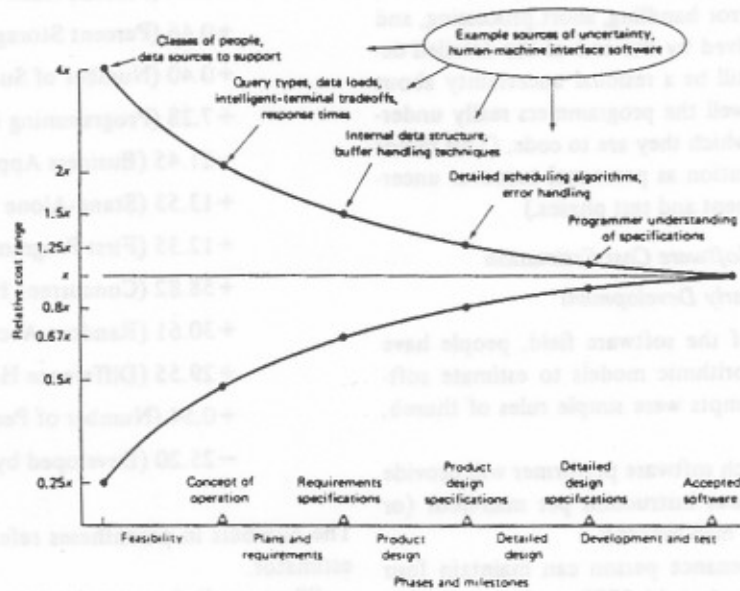
Fig. 3. Software cost estimation accuracy versus phase.
