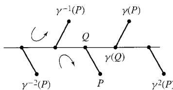
12.4 Figure Glide reflection \gamma .
