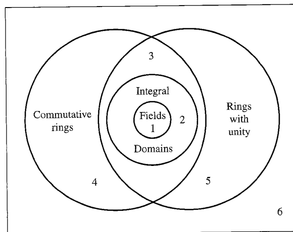
19.10 Figure A collection of rings.
