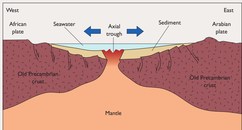
(c) GEOLOGIC (WEST-EAST) CROSS SECTION
