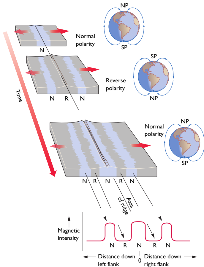
(a) MAGNETIC ANOMALY STRIPES
