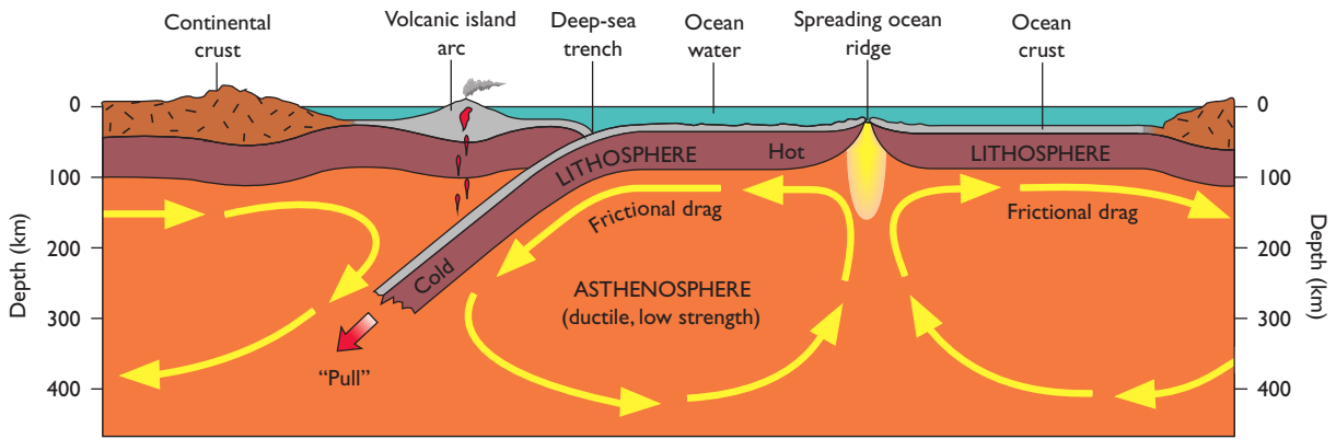
DRIVING MECHANISMS FOR PLATE MOTIONS
