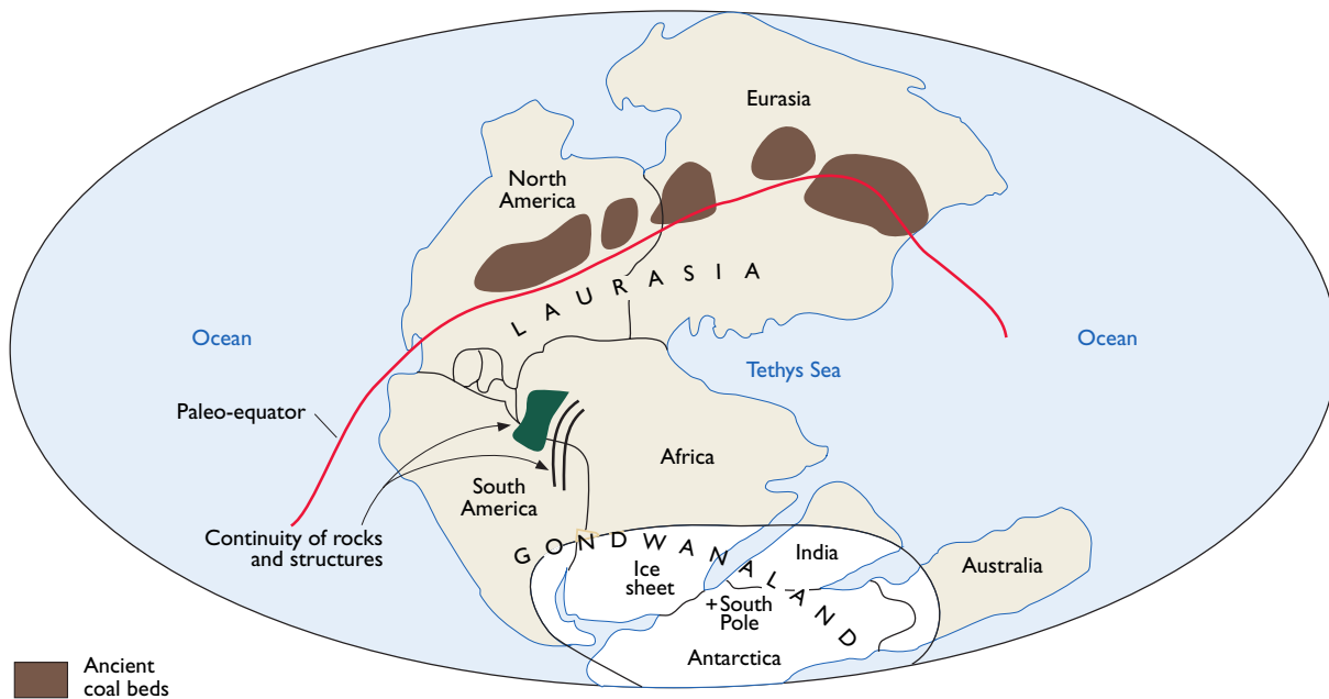
(b) PANGAEA, 200 TO 300 MYBP (MILLIONS OF YEARS BEFORE THE PRESENT)
