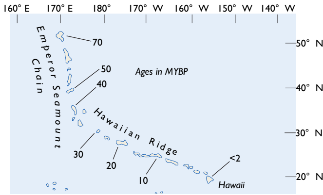
(a) VOLCANIC CHAINS
