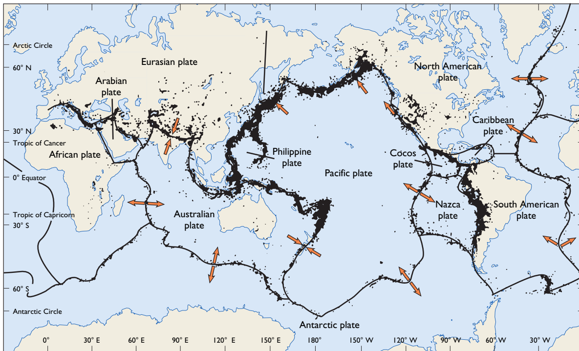
(a) LITHOSPHERIC PLATES
