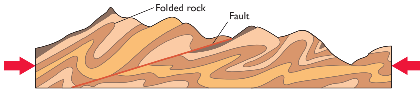
(b) SEDIMENTARY ROCKS SQUEEZED BY COMPRESSION
