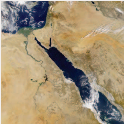
(a) SATELLITE IMAGE OF THE RED SEA REGION
