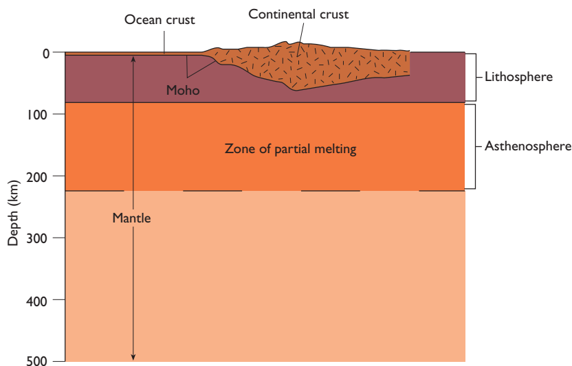
(b) THE LITHOSPHERE AND THE ASTHENOSPHERE
