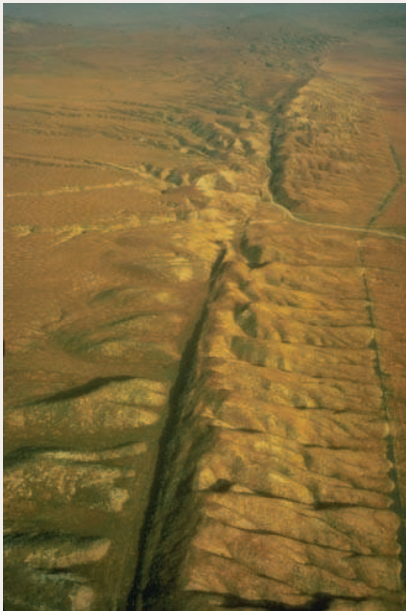
(a) SAN ANDREAS FAULT
