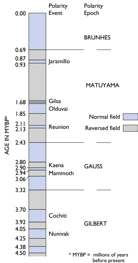
(c) GEOMAGNETIC POLARITY TIME SCALE
