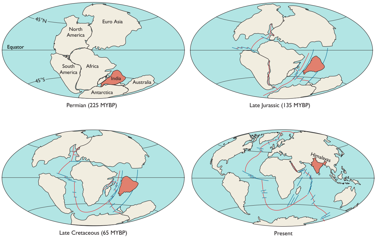
(a) THE BREAKUP OF PANGAEA
