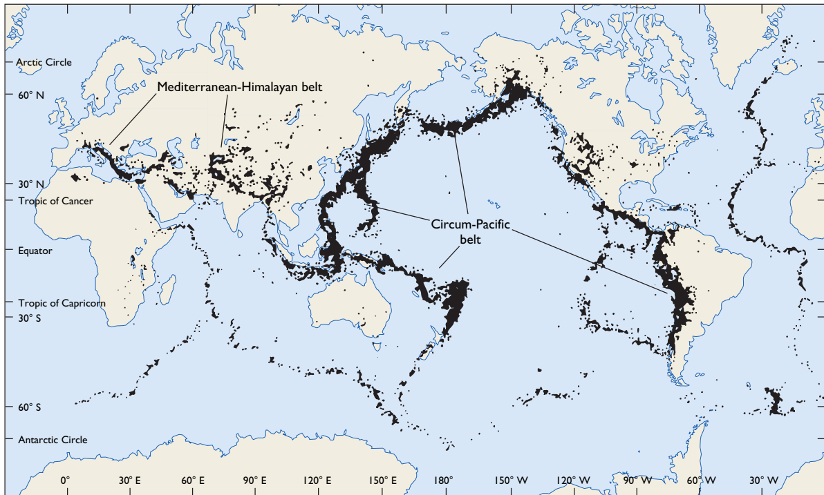
(a) GLOBAL DISTRIBUTION OF EARTHQUAKES
