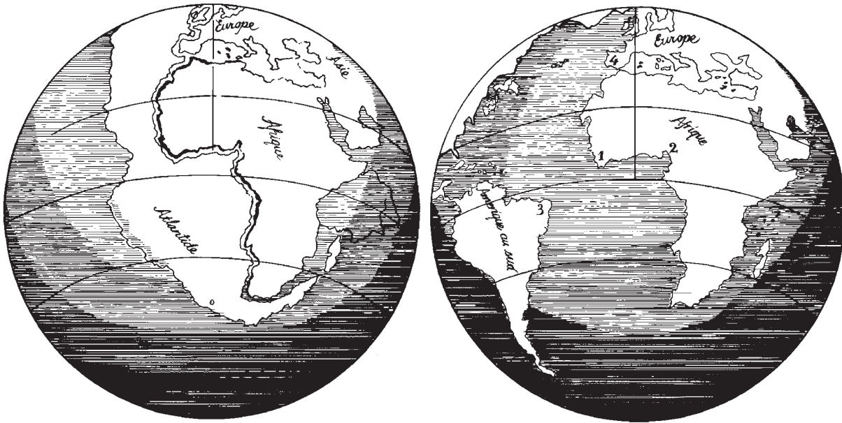
(a) FITTING THE CONTINENTS TOGETHER
