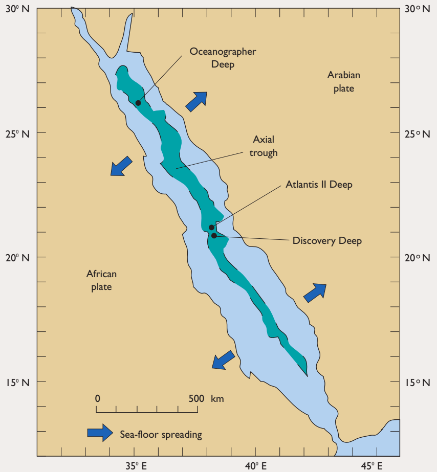
(b) THE RED SEA SPREADING CENTER
