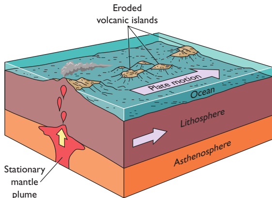
(b) MANTLE PLUME
