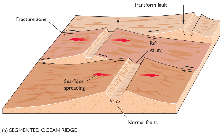
(a) SEGMENTED OCEAN RIDGE
