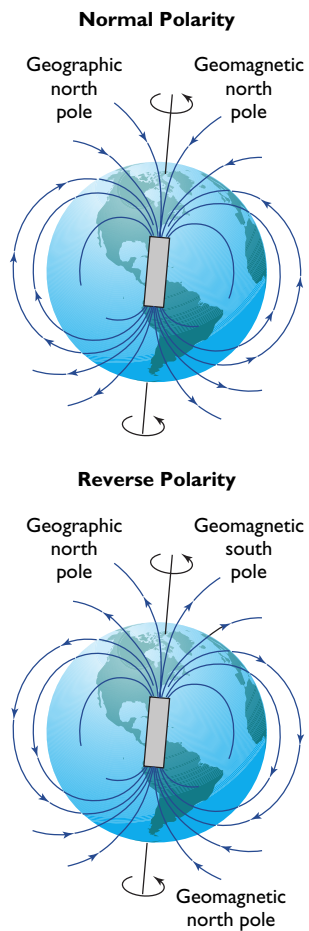
(b) GEOMAGNETIC POLARITY REVERSALS
