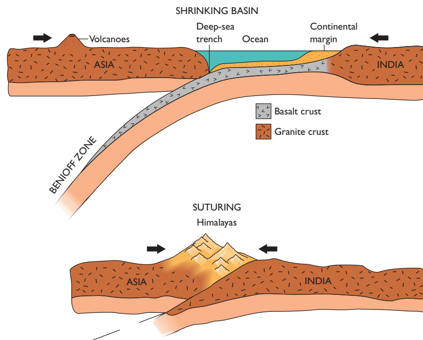
(b) PLATE TECTONIC MODEL
