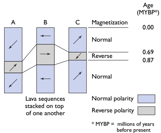
(a) MAGNETIZATION OF LAVAS
