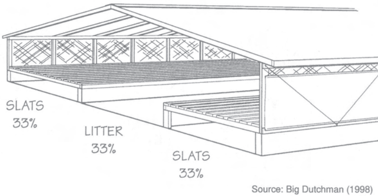
Fig. 8.10 Interior of slatted floor breeder house.
