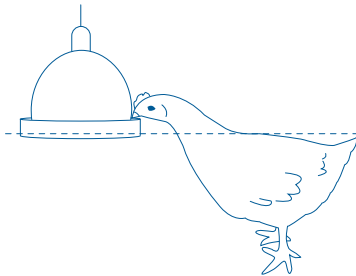
Figure 14: Height of Bell Drinker
