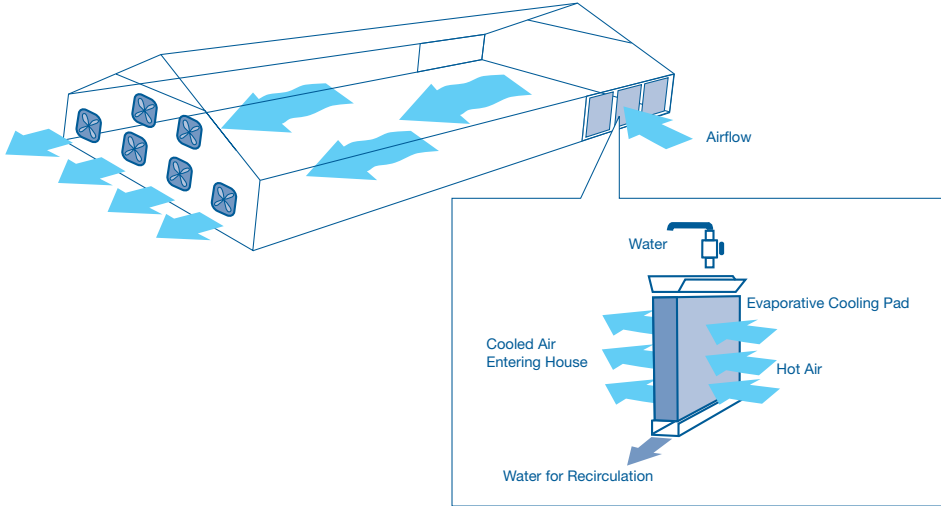
Figure 20: Pad Cooling with Tunnel Ventilation
