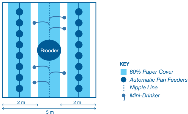
Figure 4: Typical Spot Brooding Layout (1,000 chicks)
