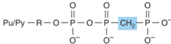
\beta,\gamma -Methylene derivative
