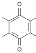
Q : Fully oxidized (quinone) form
