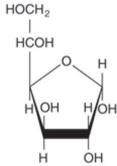
\alpha -D-Glucofuranose
