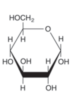
\alpha -D-Glucopyranose
