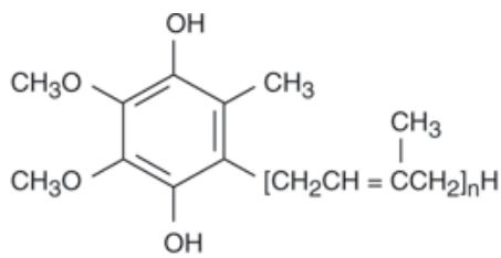
QH 2 : Reduced (quinol) form (QH 2 )
